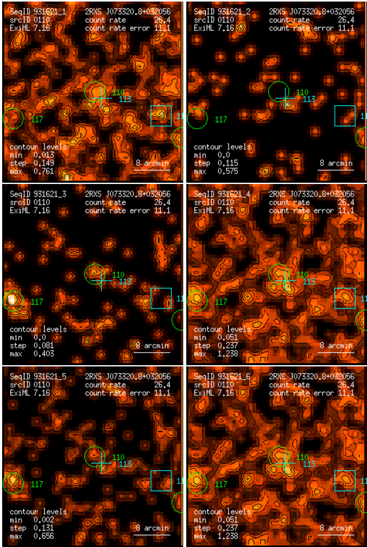
Figure 110: RASS 931621: detection 0110: band rate images, Gaussian filter: (1) PSPC channels 11 – 41, (2) 52 – 90, (3) 91 – 201, (4) 11 – 235, (5) 52 – 201, (6) 11 – 201. Broad band rates in counts/ks. Band rate contour levels in counts/ks/arcmin 2 .
