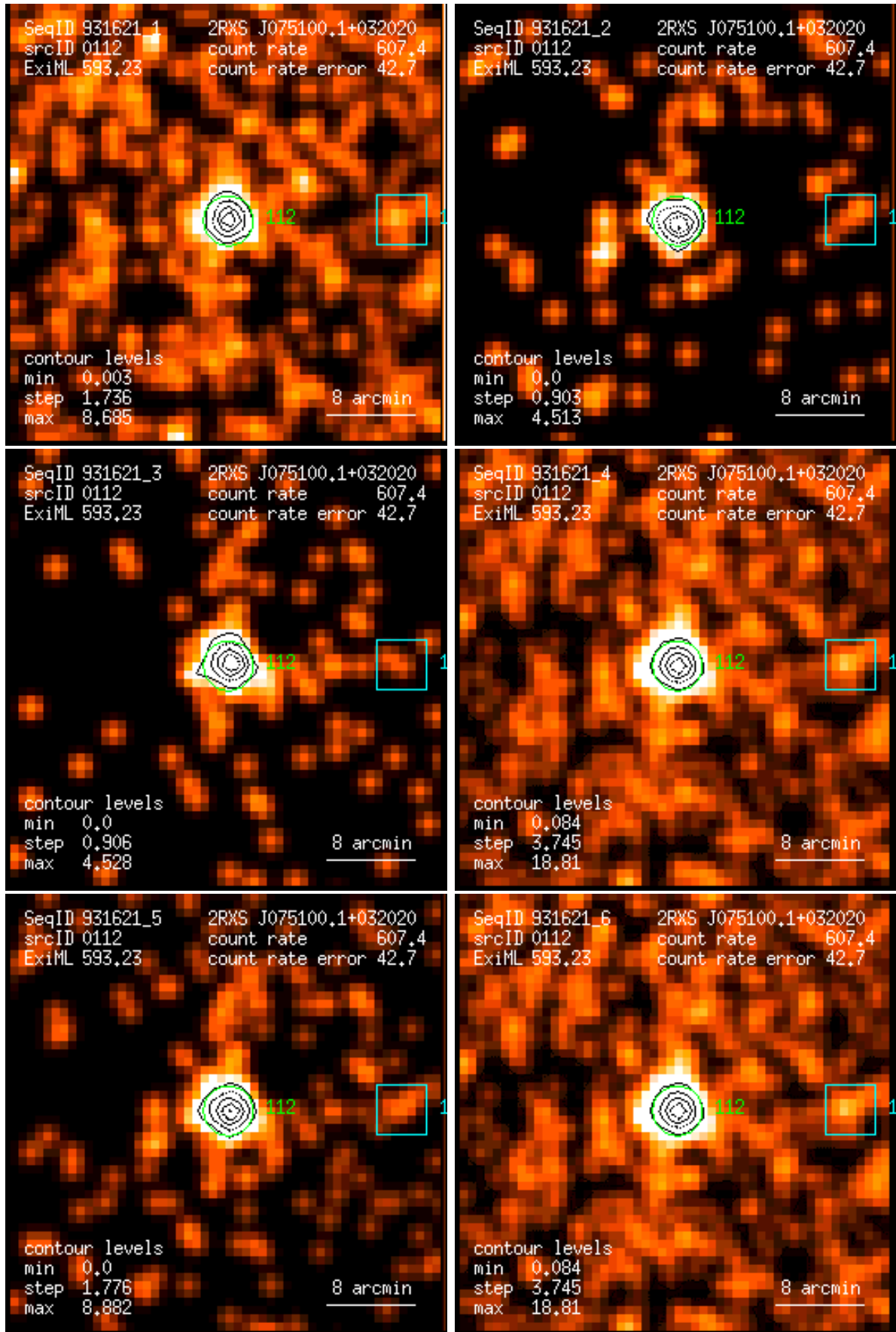
Figure 112: RASS 931621: detection 0112: band rate images, Gaussian filter: (1) PSPC channels 11 – 41, (2) 52 – 90, (3) 91 – 201, (4) 11 – 235, (5) 52 – 201, (6) 11 – 201. Broad band rates in counts/ks. Band rate contour levels in counts/ks/arcmin 2 .
