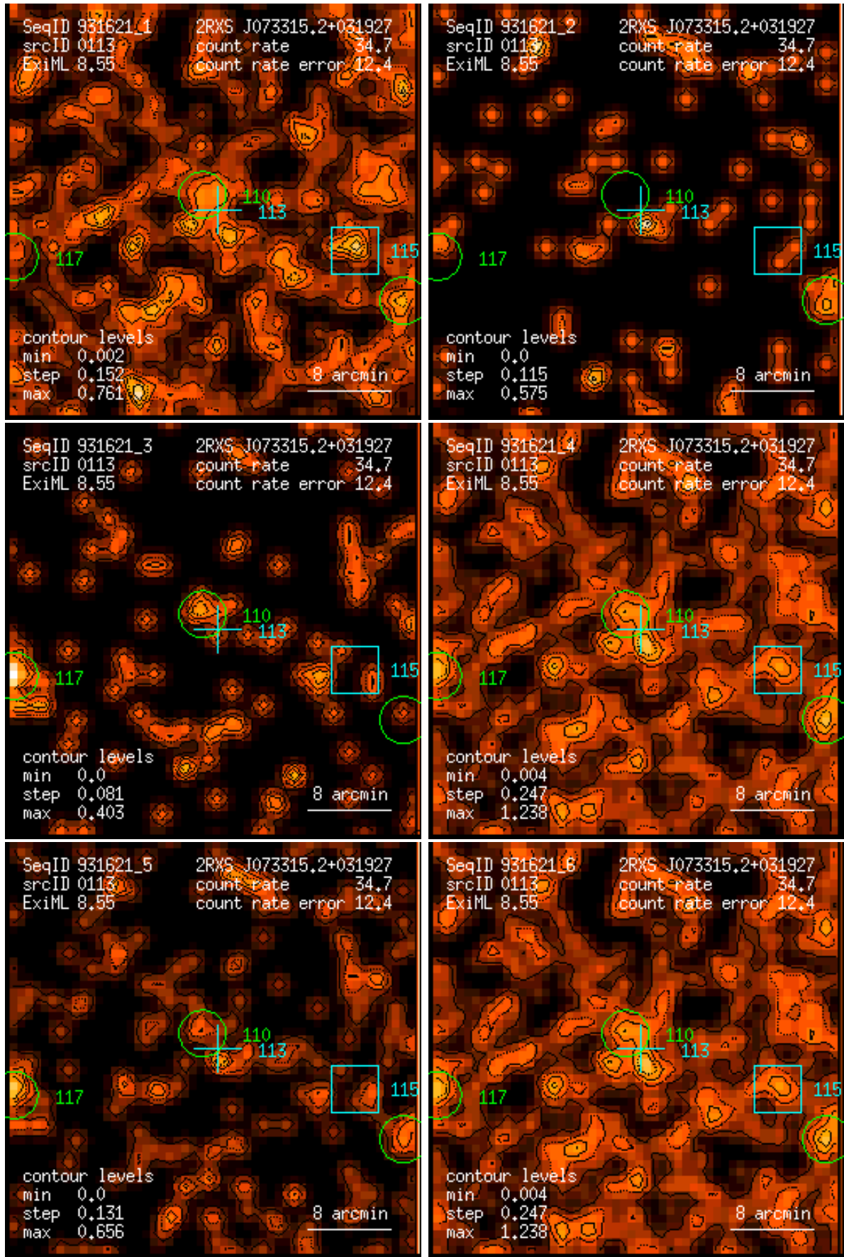
Figure 113: RASS 931621: detection 0113: band rate images, Gaussian filter: (1) PSPC channels 11 – 41, (2) 52 – 90, (3) 91 – 201, (4) 11 – 235, (5) 52 – 201, (6) 11 – 201. Broad band rates in counts/ks. Band rate contour levels in counts/ks/arcmin 2 .
