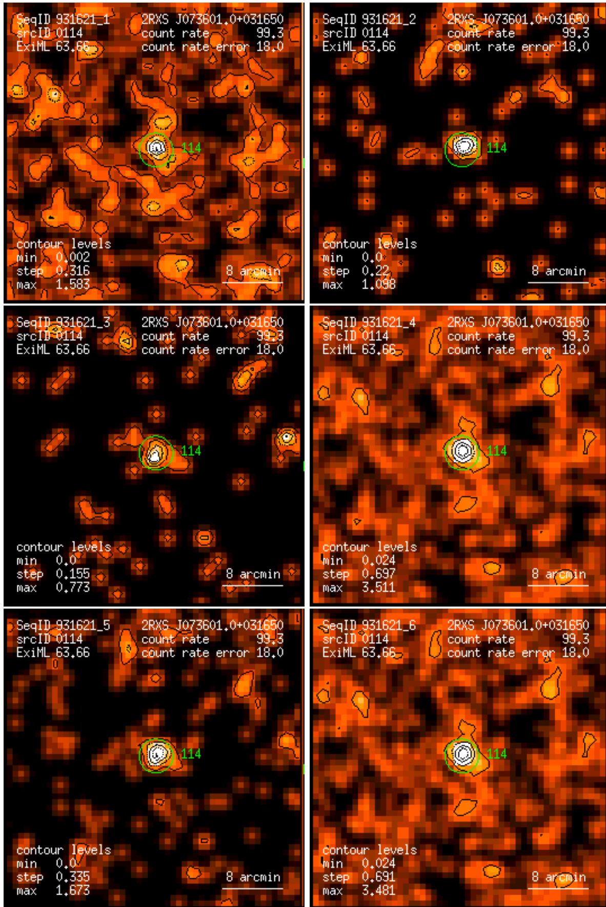
Figure 114: RASS 931621: detection 0114: band rate images, Gaussian filter: (1) PSPC channels 11 – 41, (2) 52 – 90, (3) 91 – 201, (4) 11 – 235, (5) 52 – 201, (6) 11 – 201. Broad band rates in counts/ks. Band rate contour levels in counts/ks/arcmin 2 .
