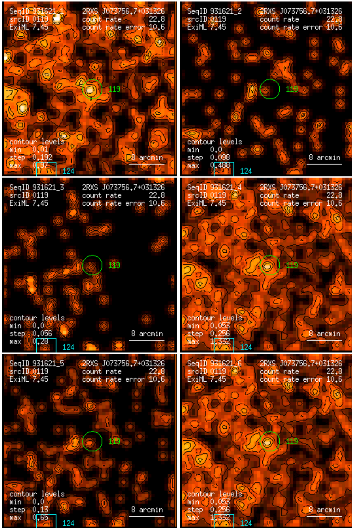
Figure 119: RASS 931621: detection 0119: band rate images, Gaussian filter: (1) PSPC channels 11 – 41, (2) 52 – 90, (3) 91 – 201, (4) 11 – 235, (5) 52 – 201, (6) 11 – 201. Broad band rates in counts/ks. Band rate contour levels in counts/ks/arcmin 2 .
