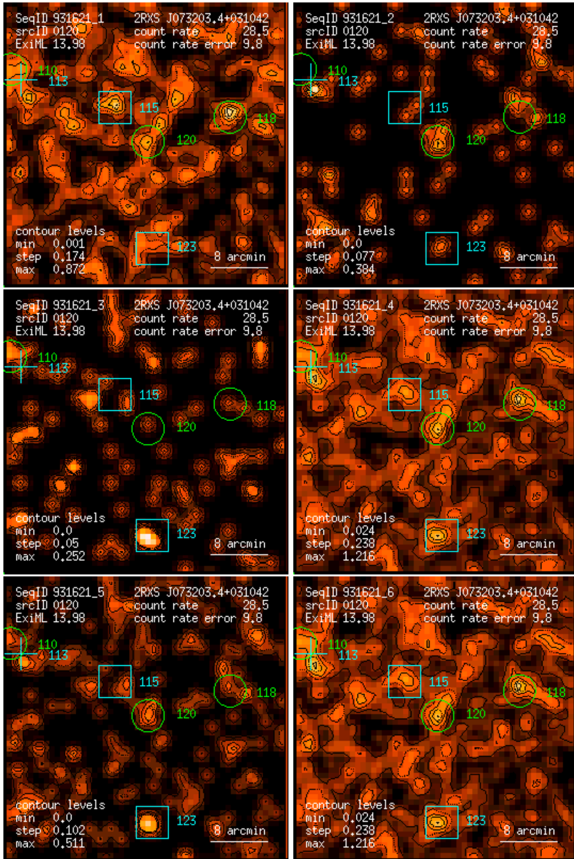
Figure 120: RASS 931621: detection 0120: band rate images, Gaussian filter: (1) PSPC channels 11 – 41, (2) 52 – 90, (3) 91 – 201, (4) 11 – 235, (5) 52 – 201, (6) 11 – 201. Broad band rates in counts/ks. Band rate contour levels in counts/ks/arcmin 2 .
