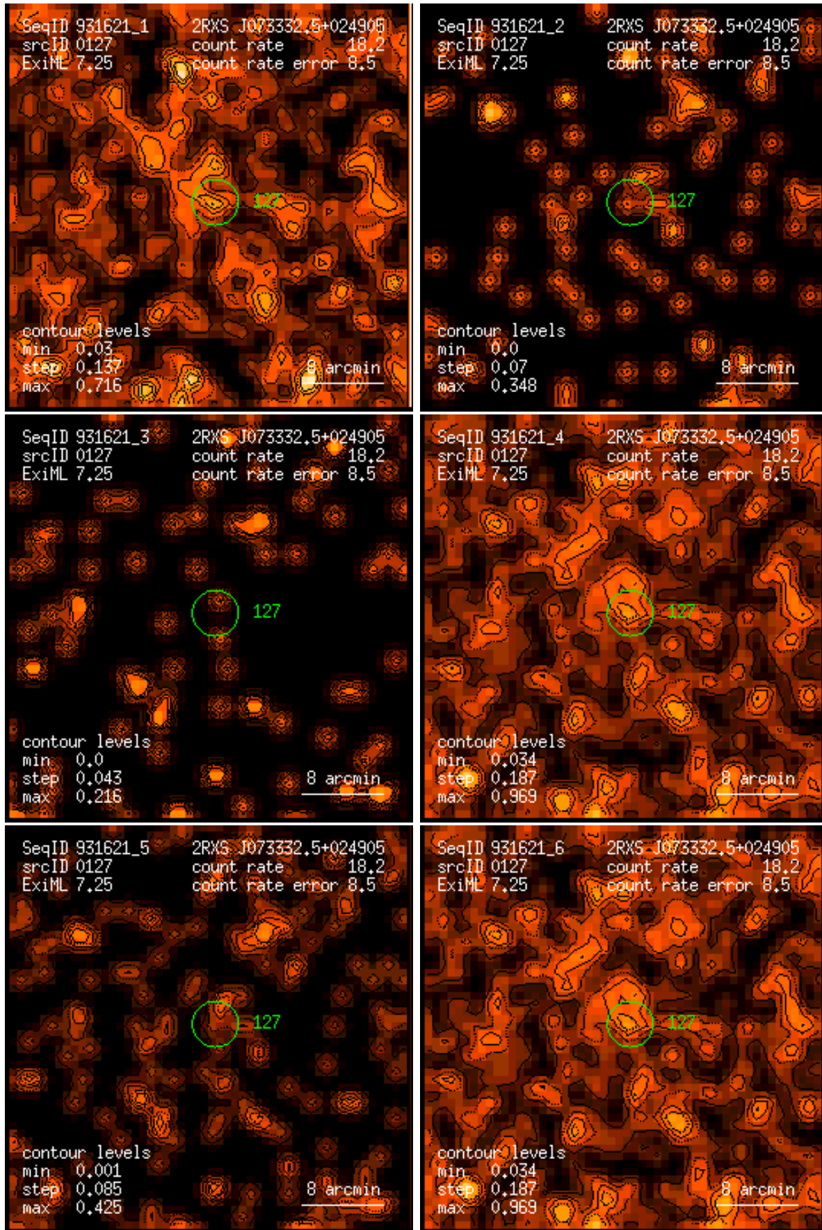
Figure 127: RASS 931621: detection 0127: band rate images, Gaussian filter: (1) PSPC channels 11 – 41, (2) 52 – 90, (3) 91 – 201, (4) 11 – 235, (5) 52 – 201, (6) 11 – 201. Broad band rates in counts/ks. Band rate contour levels in counts/ks/arcmin 2 .
