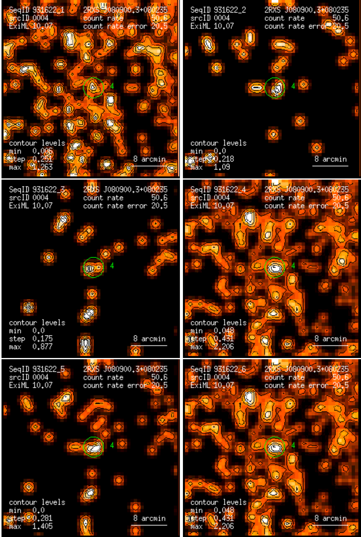
Figure 4: RASS 931622: detection 0004: band rate images, Gaussian filter: (1) PSPC channels 11 – 41, (2) 52 – 90, (3) 91 – 201, (4) 11 – 235, (5) 52 – 201, (6) 11 – 201. Broad band rates in counts/ks. Band rate contour levels in counts/ks/arcmin 2 .
