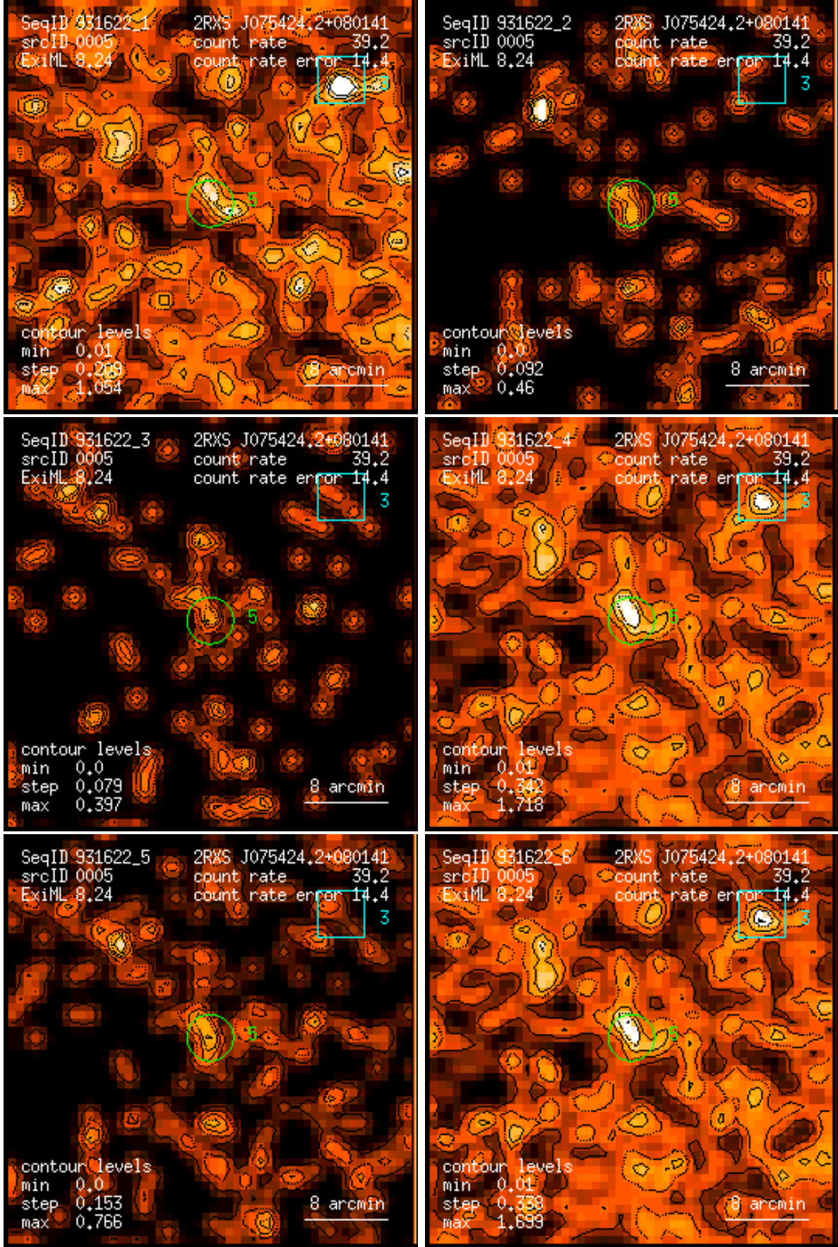
Figure 5: RASS 931622: detection 0005: band rate images, Gaussian filter: (1) PSPC channels 11 – 41, (2) 52 – 90, (3) 91 – 201, (4) 11 – 235, (5) 52 – 201, (6) 11 – 201. Broad band rates in counts/ks. Band rate contour levels in counts/ks/arcmin 2 .
