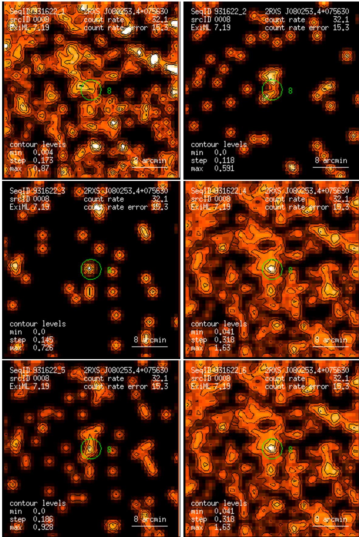
Figure 8: RASS 931622: detection 0008: band rate images, Gaussian filter: (1) PSPC channels 11 – 41, (2) 52 – 90, (3) 91 – 201, (4) 11 – 235, (5) 52 – 201, (6) 11 – 201. Broad band rates in counts/ks. Band rate contour levels in counts/ks/arcmin 2 .
