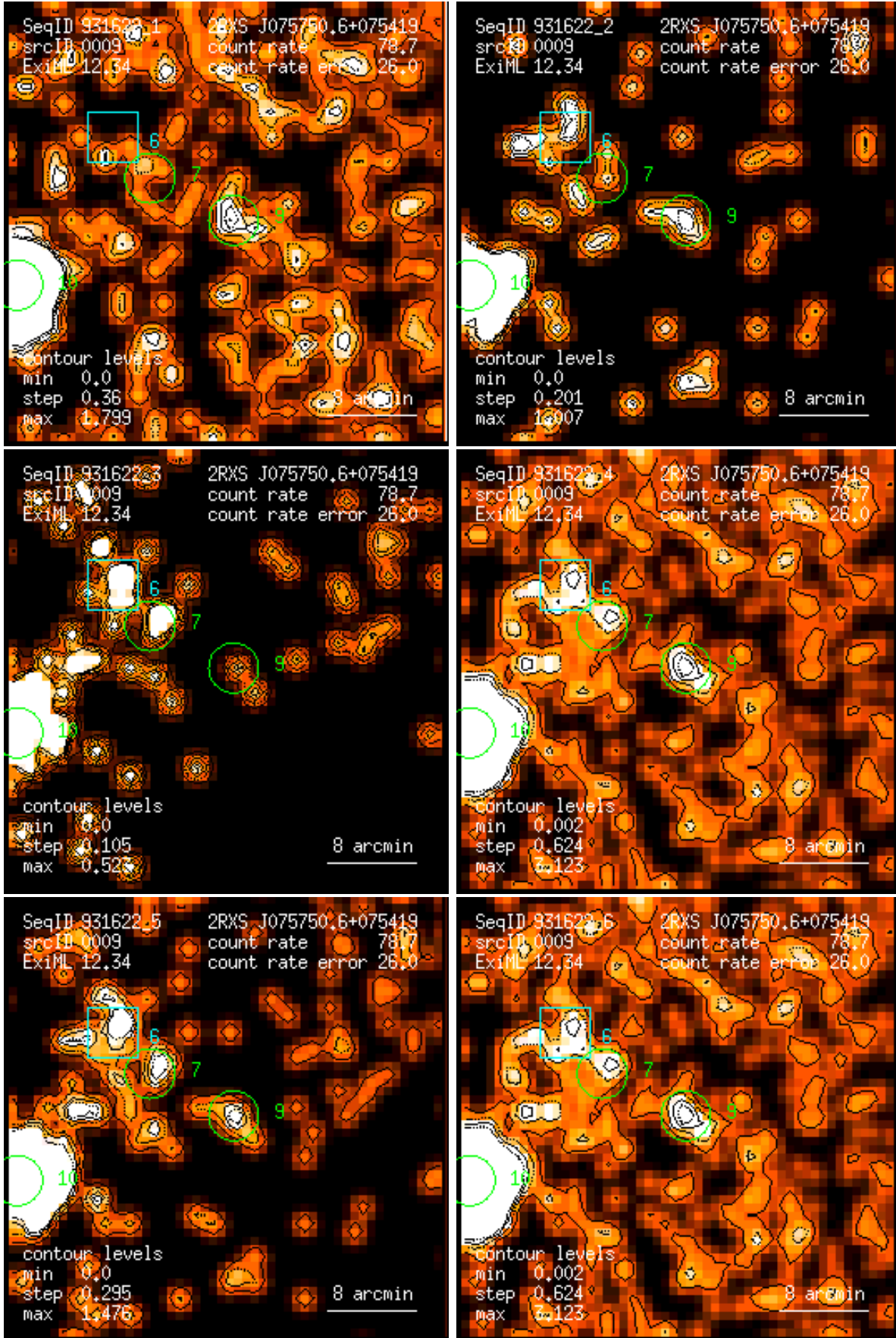
Figure 9: RASS 931622: detection 0009: band rate images, Gaussian filter: (1) PSPC channels 11 – 41, (2) 52 – 90, (3) 91 – 201, (4) 11 – 235, (5) 52 – 201, (6) 11 – 201. Broad band rates in counts/ks. Band rate contour levels in counts/ks/arcmin 2 .
