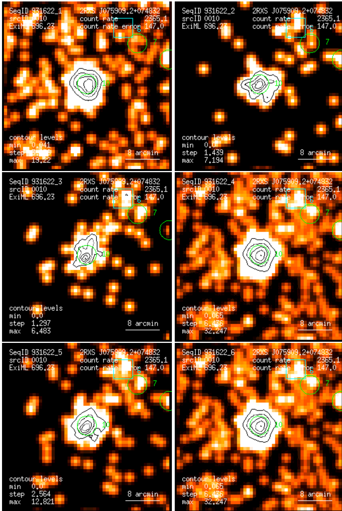
Figure 10: RASS 931622: detection 0010: band rate images, Gaussian filter: (1) PSPC channels 11 – 41, (2) 52 – 90, (3) 91 – 201, (4) 11 – 235, (5) 52 – 201, (6) 11 – 201. Broad band rates in counts/ks. Band rate contour levels in counts/ks/arcmin 2 .
