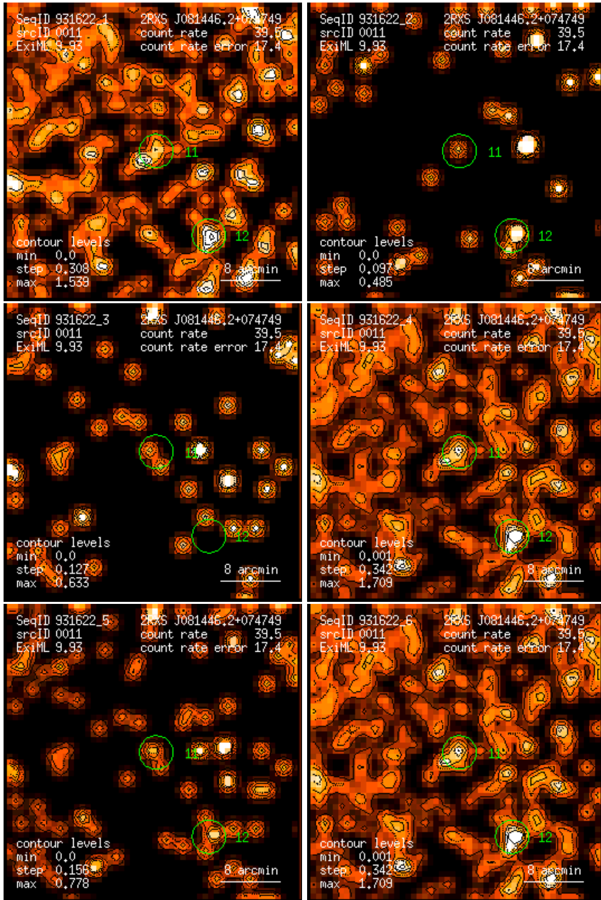
Figure 11: RASS 931622: detection 0011: band rate images, Gaussian filter: (1) PSPC channels 11 – 41, (2) 52 – 90, (3) 91 – 201, (4) 11 – 235, (5) 52 – 201, (6) 11 – 201. Broad band rates in counts/ks. Band rate contour levels in counts/ks/arcmin 2 .
