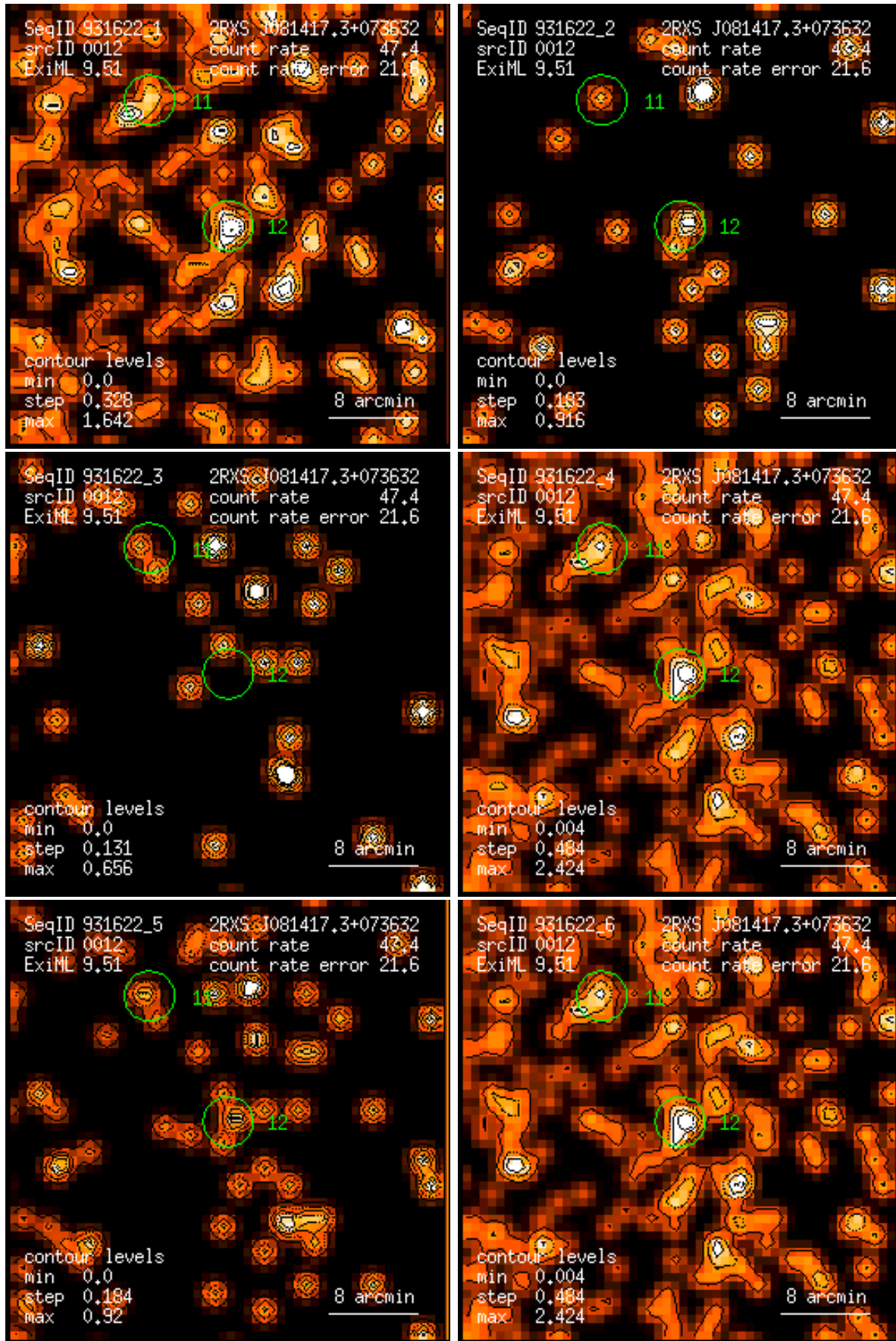
Figure 12: RASS 931622: detection 0012: band rate images, Gaussian filter: (1) PSPC channels 11 – 41, (2) 52 – 90, (3) 91 – 201, (4) 11 – 235, (5) 52 – 201, (6) 11 – 201. Broad band rates in counts/ks. Band rate contour levels in counts/ks/arcmin 2 .
