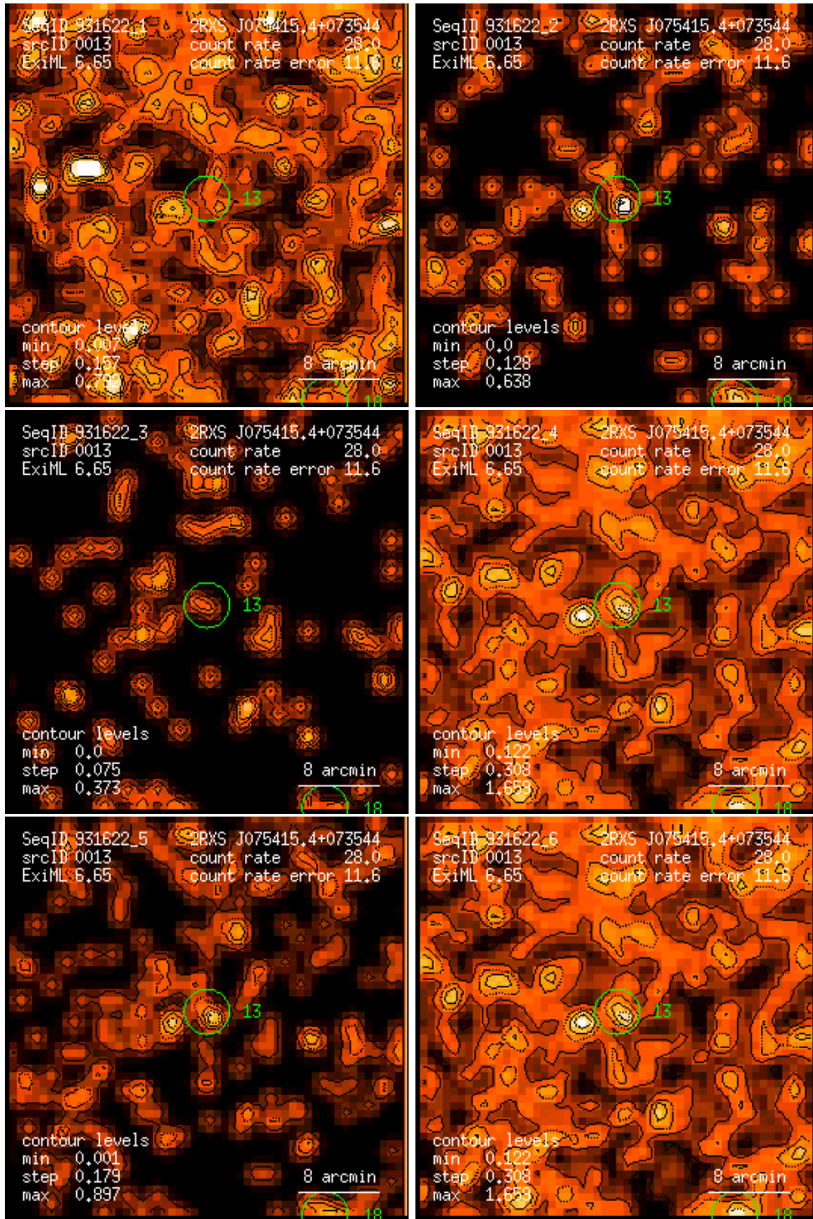
Figure 13: RASS 931622: detection 0013: band rate images, Gaussian filter: (1) PSPC channels 11 – 41, (2) 52 – 90, (3) 91 – 201, (4) 11 – 235, (5) 52 – 201, (6) 11 – 201. Broad band rates in counts/ks. Band rate contour levels in counts/ks/arcmin 2 .
