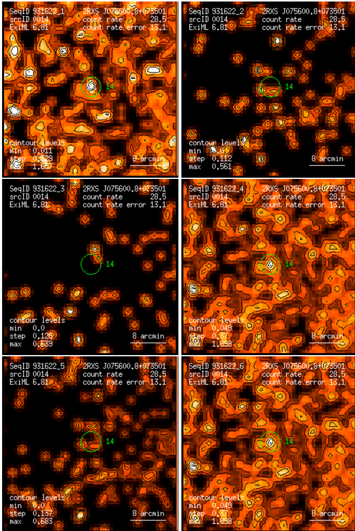
Figure 14: RASS 931622: detection 0014: band rate images, Gaussian filter: (1) PSPC channels 11 – 41, (2) 52 – 90, (3) 91 – 201, (4) 11 – 235, (5) 52 – 201, (6) 11 – 201. Broad band rates in counts/ks. Band rate contour levels in counts/ks/arcmin 2 .
