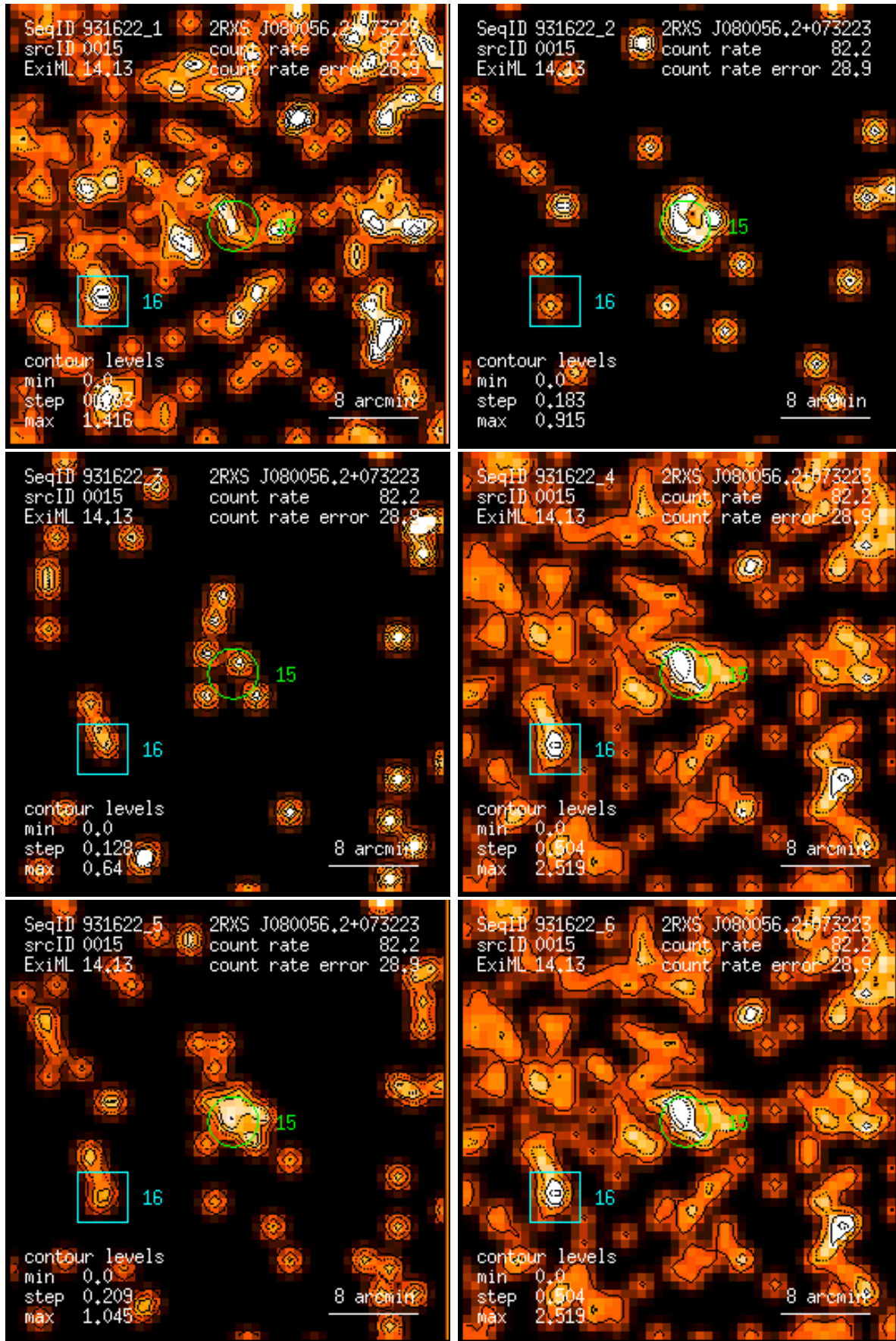
Figure 15: RASS 931622: detection 0015: band rate images, Gaussian filter: (1) PSPC channels 11 – 41, (2) 52 – 90, (3) 91 – 201, (4) 11 – 235, (5) 52 – 201, (6) 11 – 201. Broad band rates in counts/ks. Band rate contour levels in counts/ks/arcmin 2 .
