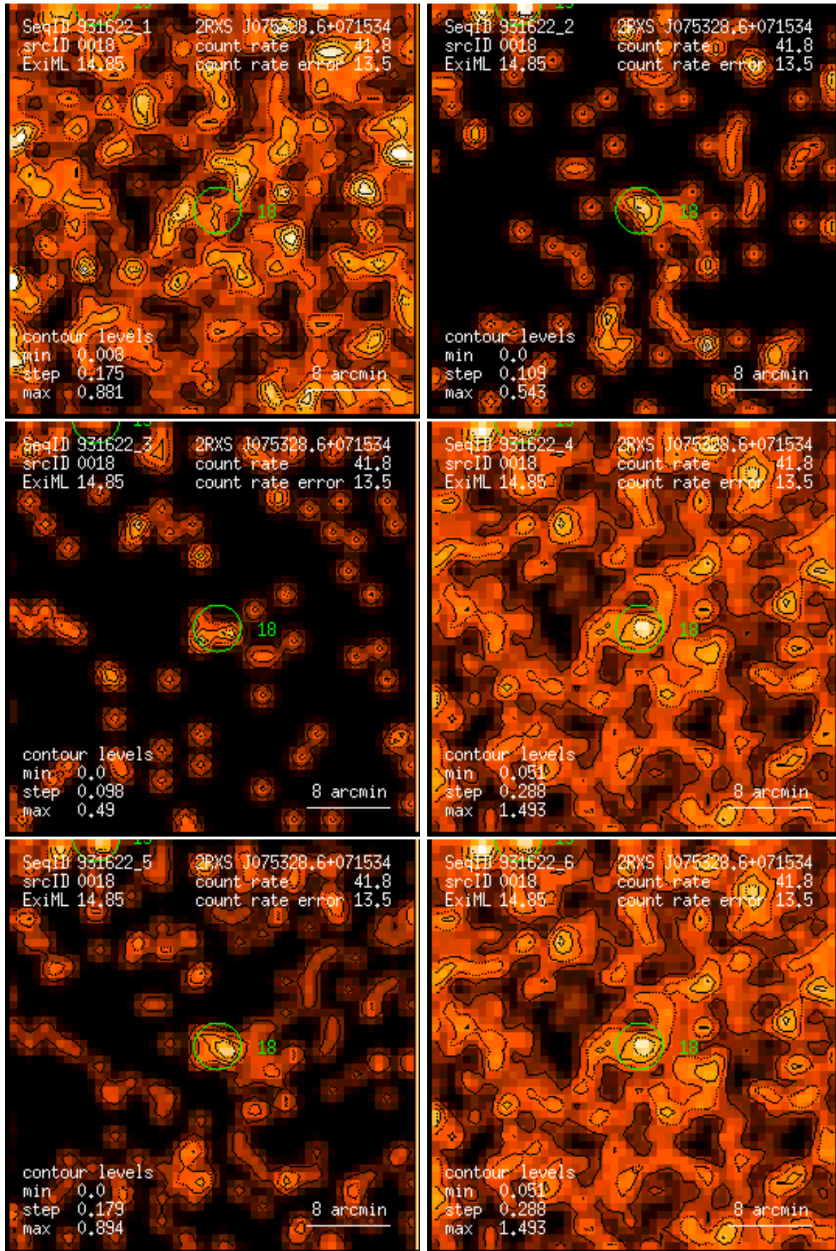
Figure 18: RASS 931622: detection 0018: band rate images, Gaussian filter: (1) PSPC channels 11 – 41, (2) 52 – 90, (3) 91 – 201, (4) 11 – 235, (5) 52 – 201, (6) 11 – 201. Broad band rates in counts/ks. Band rate contour levels in counts/ks/arcmin 2 .
