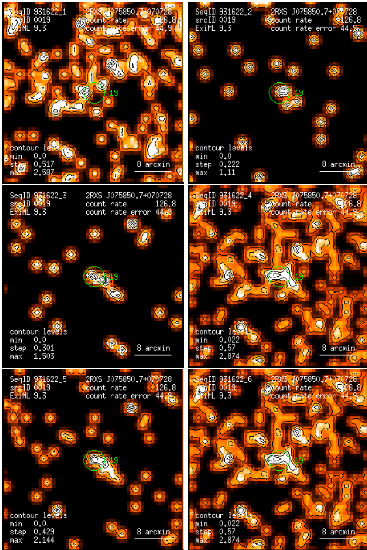
Figure 19: RASS 931622: detection 0019: band rate images, Gaussian filter: (1) PSPC channels 11 – 41, (2) 52 – 90, (3) 91 – 201, (4) 11 – 235, (5) 52 – 201, (6) 11 – 201. Broad band rates in counts/ks. Band rate contour levels in counts/ks/arcmin 2 .
