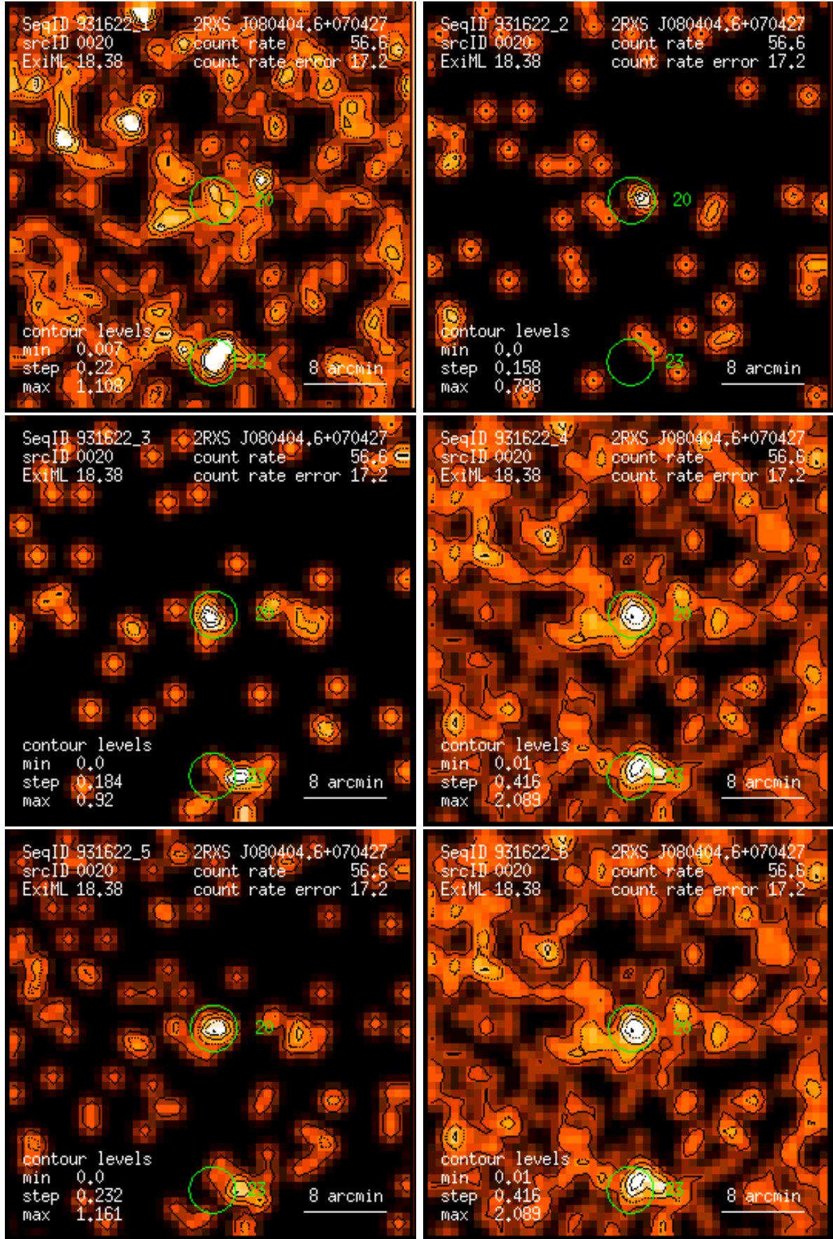
Figure 20: RASS 931622: detection 0020: band rate images, Gaussian filter: (1) PSPC channels 11 – 41, (2) 52 – 90, (3) 91 – 201, (4) 11 – 235, (5) 52 – 201, (6) 11 – 201. Broad band rates in counts/ks. Band rate contour levels in counts/ks/arcmin 2 .
