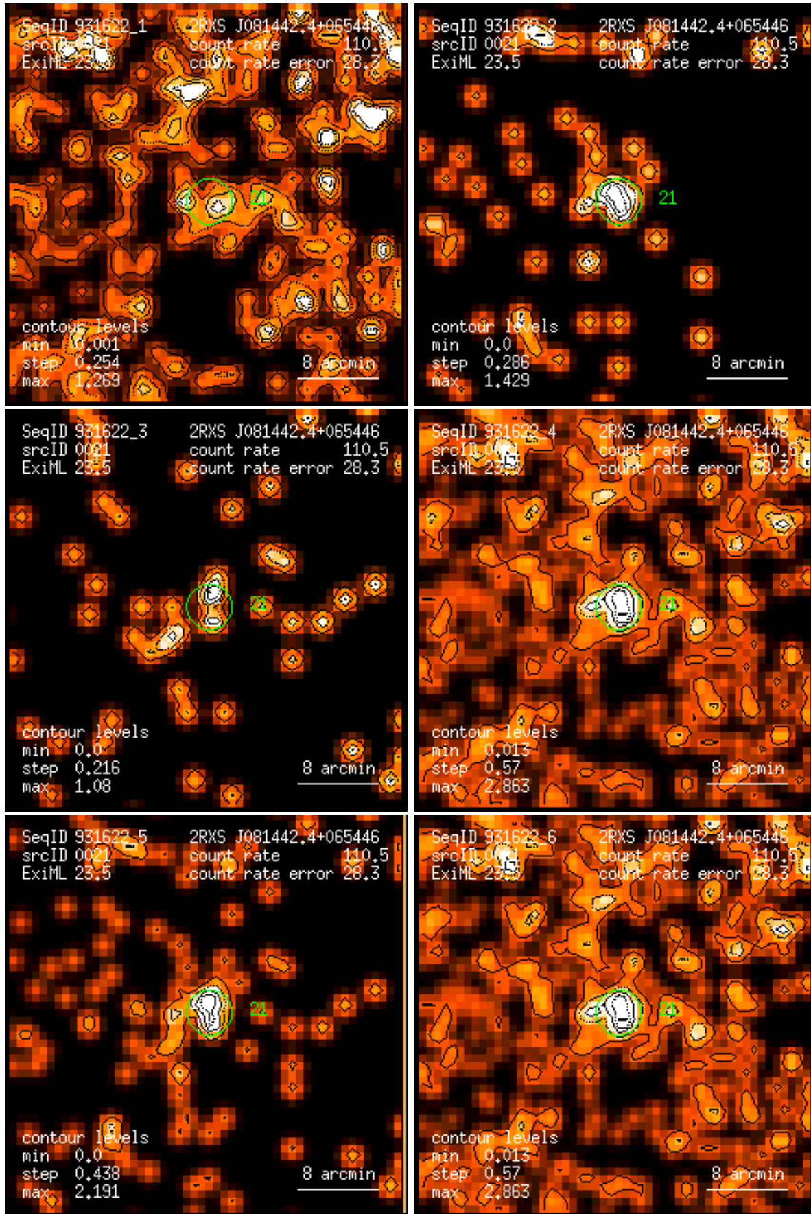
Figure 21: RASS 931622: detection 0021: band rate images, Gaussian filter: (1) PSPC channels 11 – 41, (2) 52 – 90, (3) 91 – 201, (4) 11 – 235, (5) 52 – 201, (6) 11 – 201. Broad band rates in counts/ks. Band rate contour levels in counts/ks/arcmin 2 .
