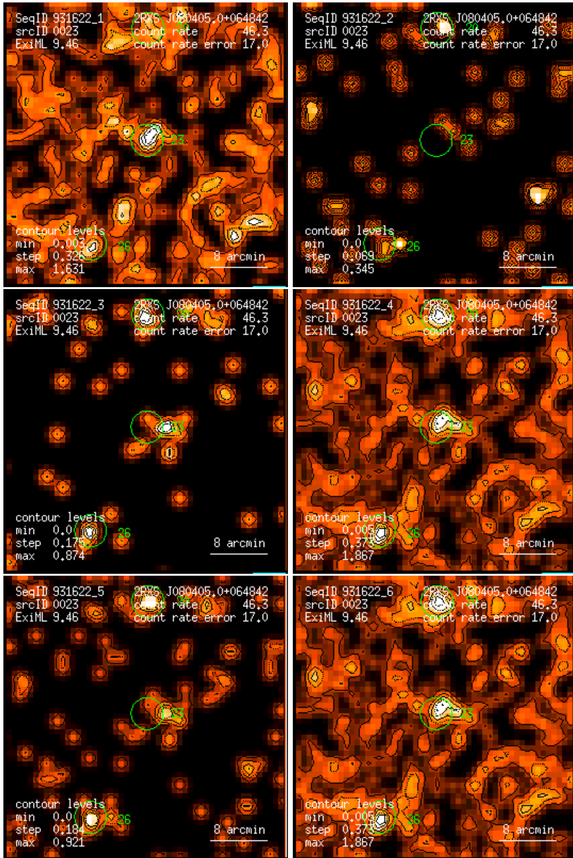
Figure 23: RASS 931622: detection 0023: band rate images, Gaussian filter: (1) PSPC channels 11 – 41, (2) 52 – 90, (3) 91 – 201, (4) 11 – 235, (5) 52 – 201, (6) 11 – 201. Broad band rates in counts/ks. Band rate contour levels in counts/ks/arcmin 2 .
