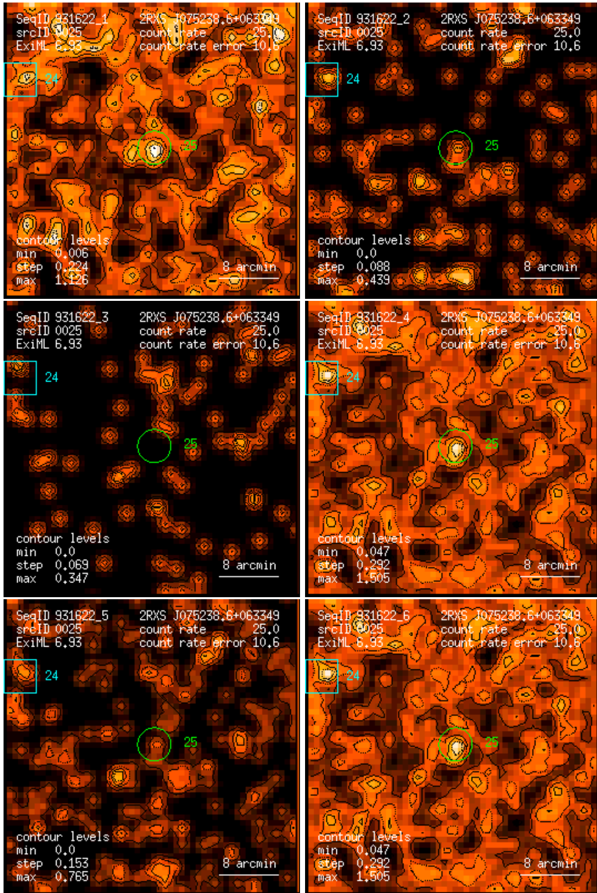
Figure 25: RASS 931622: detection 0025: band rate images, Gaussian filter: (1) PSPC channels 11 – 41, (2) 52 – 90, (3) 91 – 201, (4) 11 – 235, (5) 52 – 201, (6) 11 – 201. Broad band rates in counts/ks. Band rate contour levels in counts/ks/arcmin 2 .
