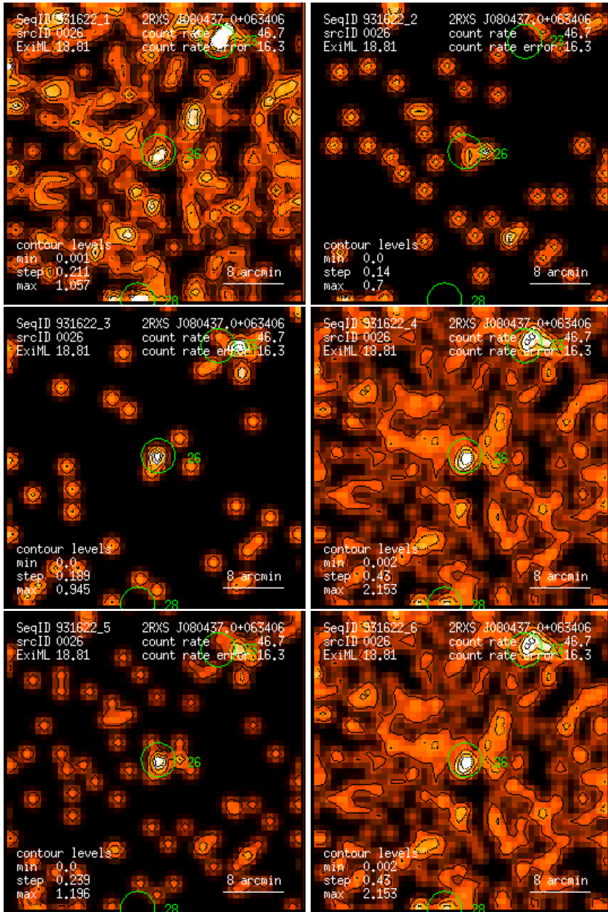
Figure 26: RASS 931622: detection 0026: band rate images, Gaussian filter: (1) PSPC channels 11 – 41, (2) 52 – 90, (3) 91 – 201, (4) 11 – 235, (5) 52 – 201, (6) 11 – 201. Broad band rates in counts/ks. Band rate contour levels in counts/ks/arcmin 2 .
