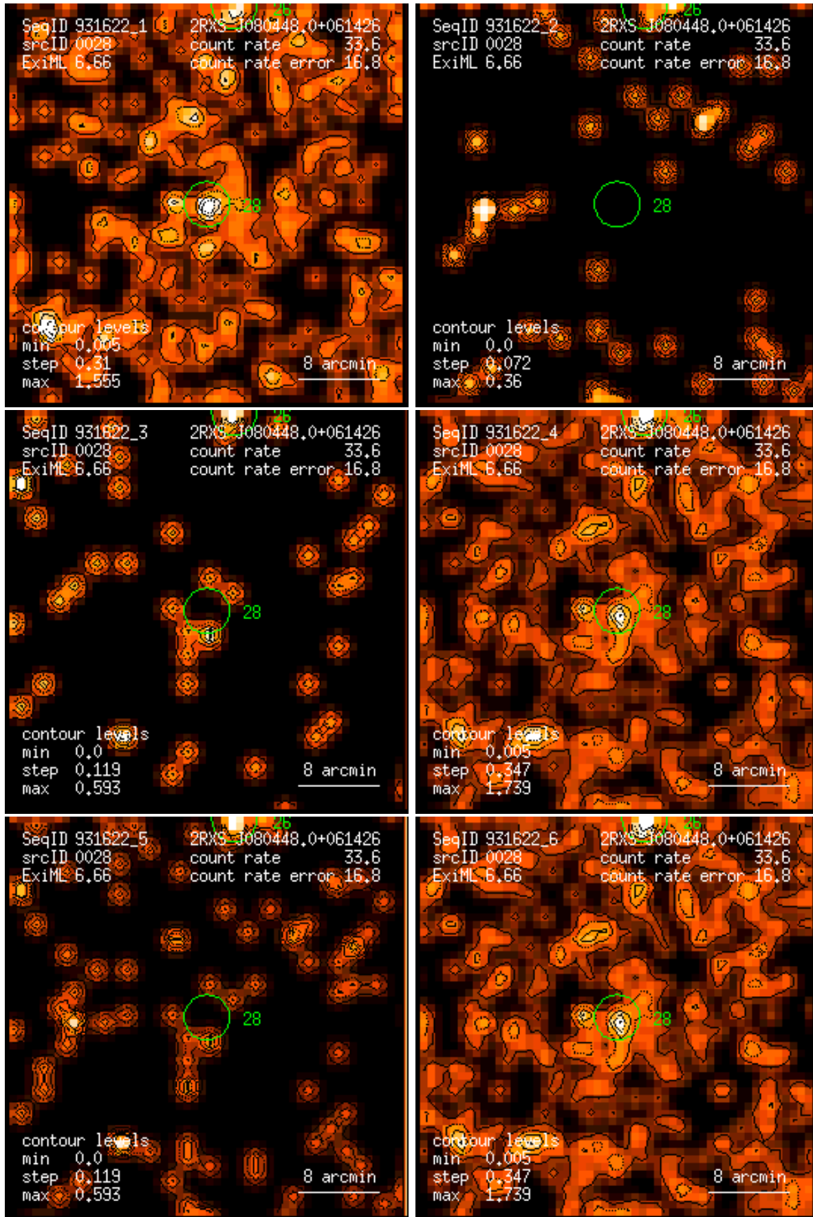
Figure 28: RASS 931622: detection 0028: band rate images, Gaussian filter: (1) PSPC channels 11 – 41, (2) 52 – 90, (3) 91 – 201, (4) 11 – 235, (5) 52 – 201, (6) 11 – 201. Broad band rates in counts/ks. Band rate contour levels in counts/ks/arcmin 2 .
