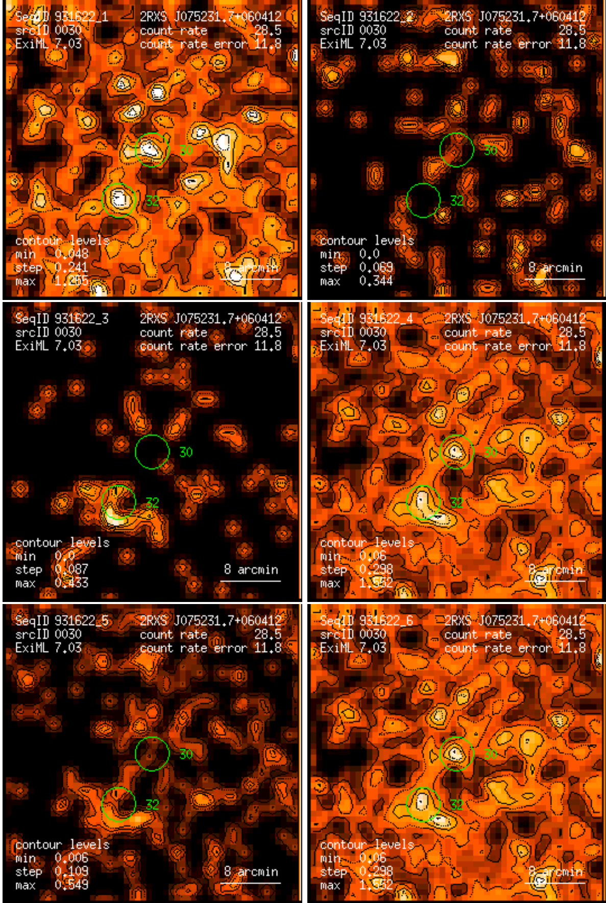
Figure 30: RASS 931622: detection 0030: band rate images, Gaussian filter: (1) PSPC channels 11 – 41, (2) 52 – 90, (3) 91 – 201, (4) 11 – 235, (5) 52 – 201, (6) 11 – 201. Broad band rates in counts/ks. Band rate contour levels in counts/ks/arcmin 2 .
