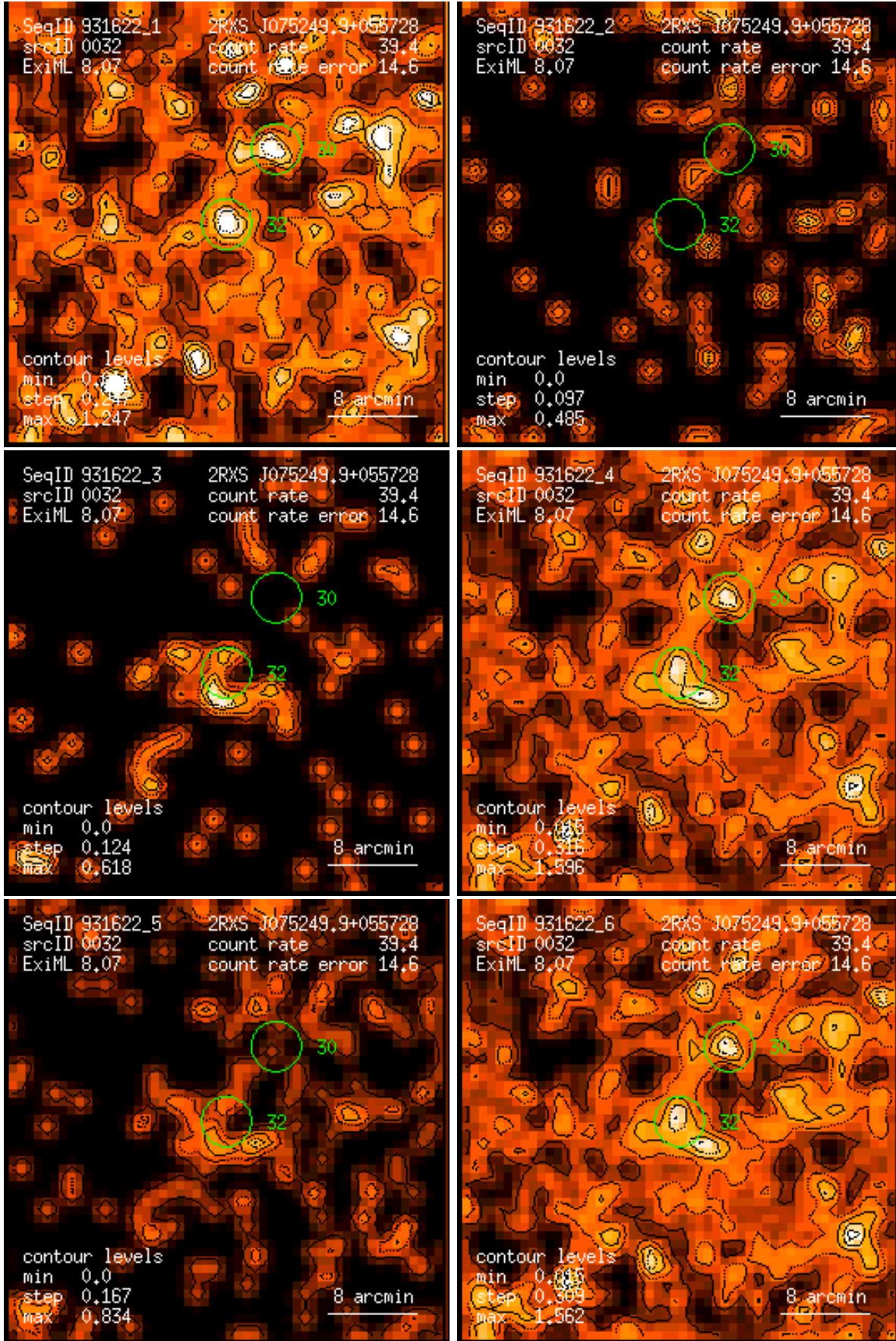
Figure 32: RASS 931622: detection 0032: band rate images, Gaussian filter: (1) PSPC channels 11 – 41, (2) 52 – 90, (3) 91 – 201, (4) 11 – 235, (5) 52 – 201, (6) 11 – 201. Broad band rates in counts/ks. Band rate contour levels in counts/ks/arcmin 2 .
