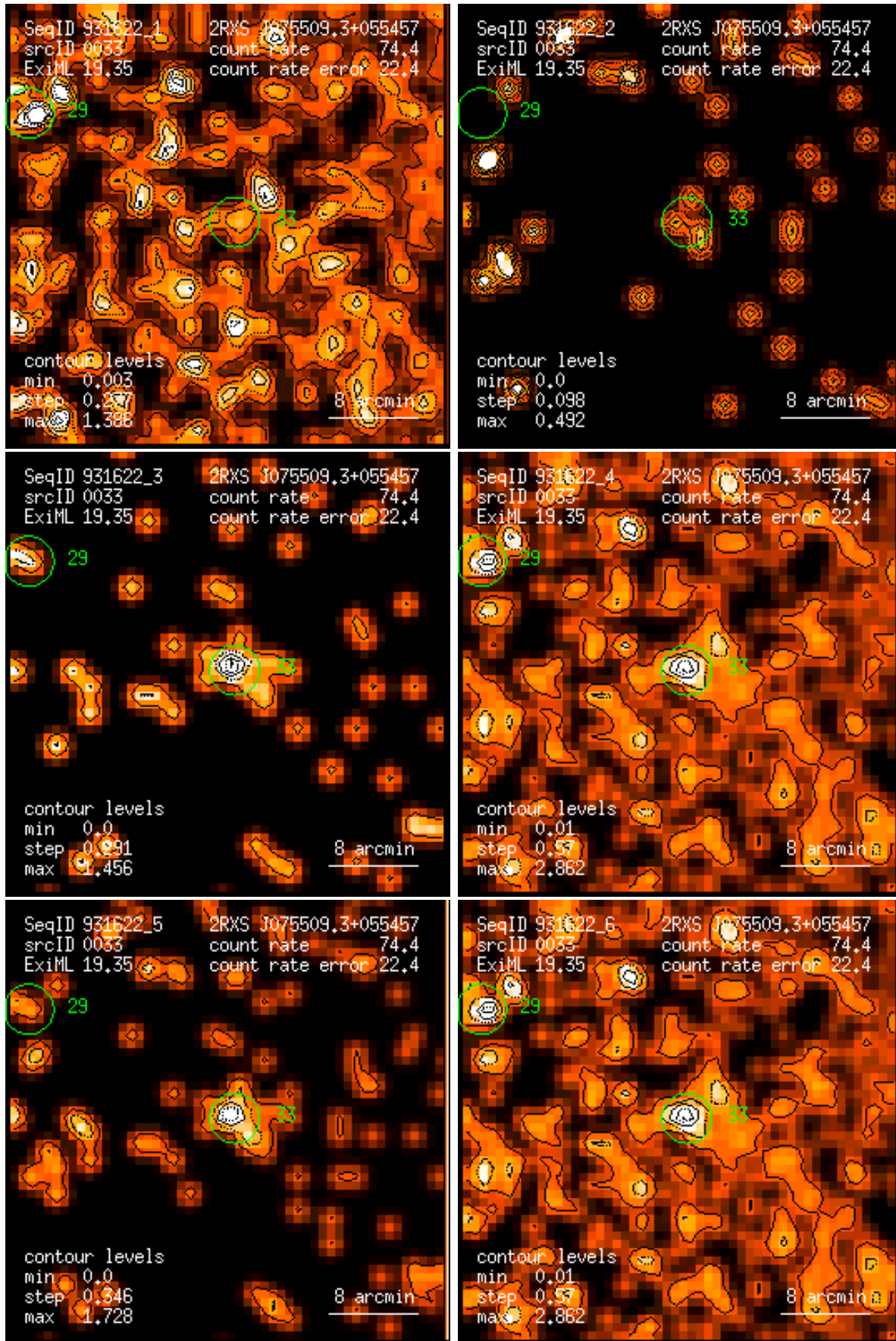
Figure 33: RASS 931622: detection 0033: band rate images, Gaussian filter: (1) PSPC channels 11 – 41, (2) 52 – 90, (3) 91 – 201, (4) 11 – 235, (5) 52 – 201, (6) 11 – 201. Broad band rates in counts/ks. Band rate contour levels in counts/ks/arcmin 2 .
