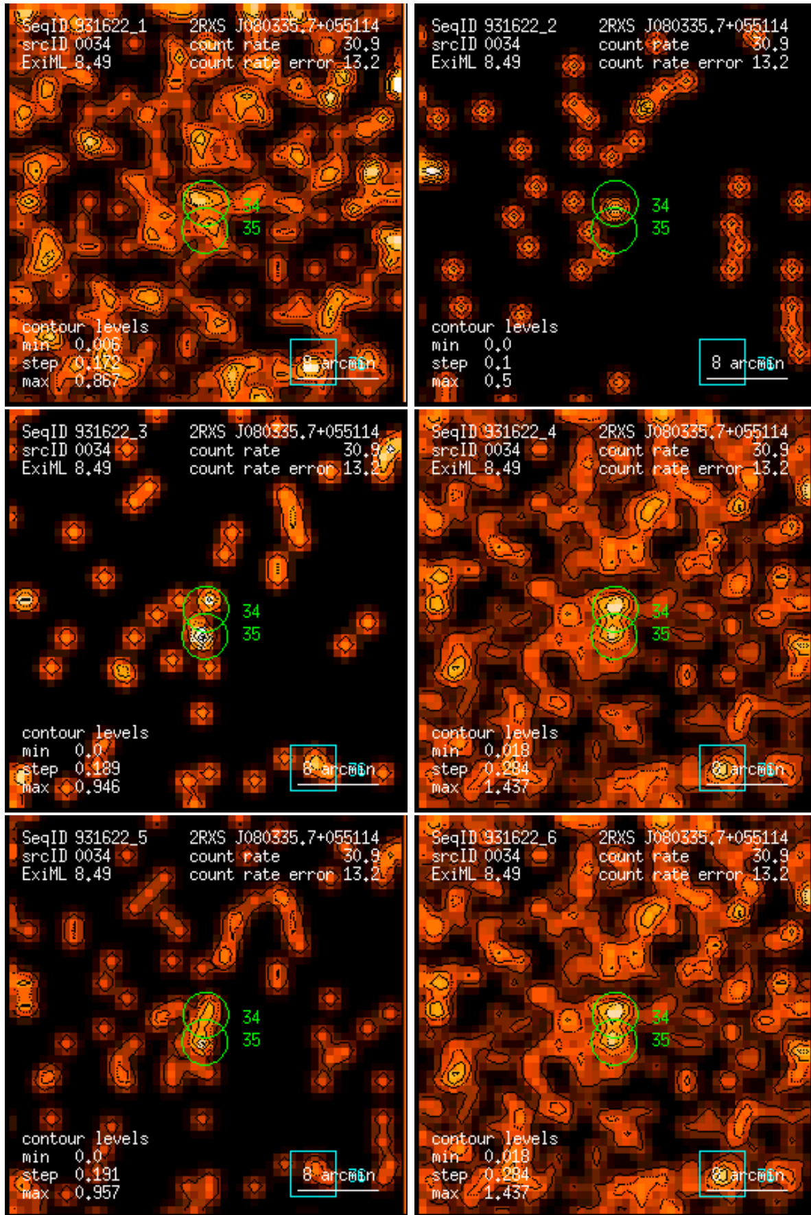
Figure 34: RASS 931622: detection 0034: band rate images, Gaussian filter: (1) PSPC channels 11 – 41, (2) 52 – 90, (3) 91 – 201, (4) 11 – 235, (5) 52 – 201, (6) 11 – 201. Broad band rates in counts/ks. Band rate contour levels in counts/ks/arcmin 2 .
