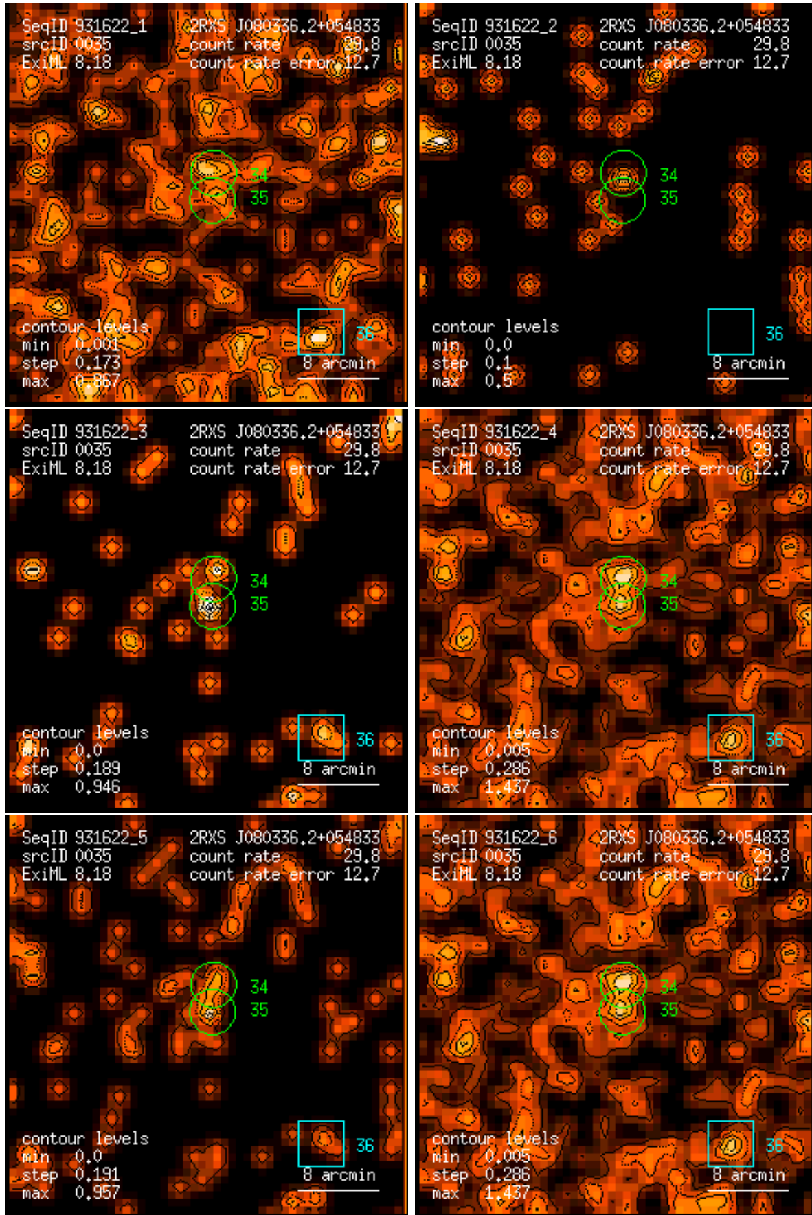
Figure 35: RASS 931622: detection 0035: band rate images, Gaussian filter: (1) PSPC channels 11 – 41, (2) 52 – 90, (3) 91 – 201, (4) 11 – 235, (5) 52 – 201, (6) 11 – 201. Broad band rates in counts/ks. Band rate contour levels in counts/ks/arcmin 2 .
