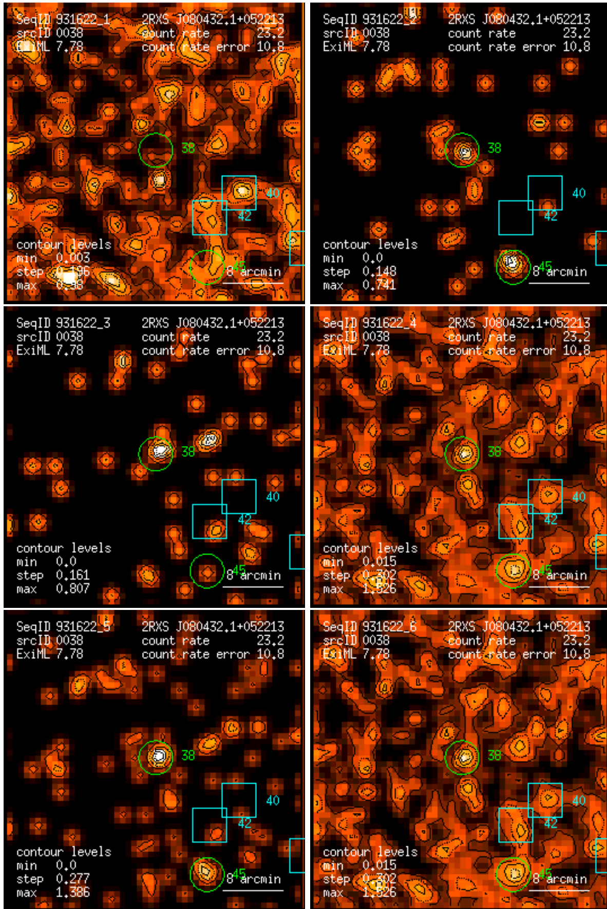
Figure 38: RASS 931622: detection 0038: band rate images, Gaussian filter: (1) PSPC channels 11 – 41, (2) 52 – 90, (3) 91 – 201, (4) 11 – 235, (5) 52 – 201, (6) 11 – 201. Broad band rates in counts/ks. Band rate contour levels in counts/ks/arcmin 2 .
