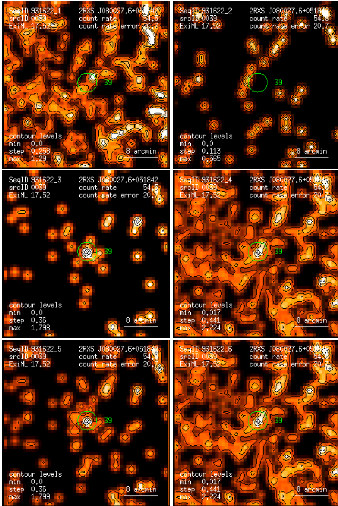
Figure 39: RASS 931622: detection 0039: band rate images, Gaussian filter: (1) PSPC channels 11 – 41, (2) 52 – 90, (3) 91 – 201, (4) 11 – 235, (5) 52 – 201, (6) 11 – 201. Broad band rates in counts/ks. Band rate contour levels in counts/ks/arcmin 2 .
