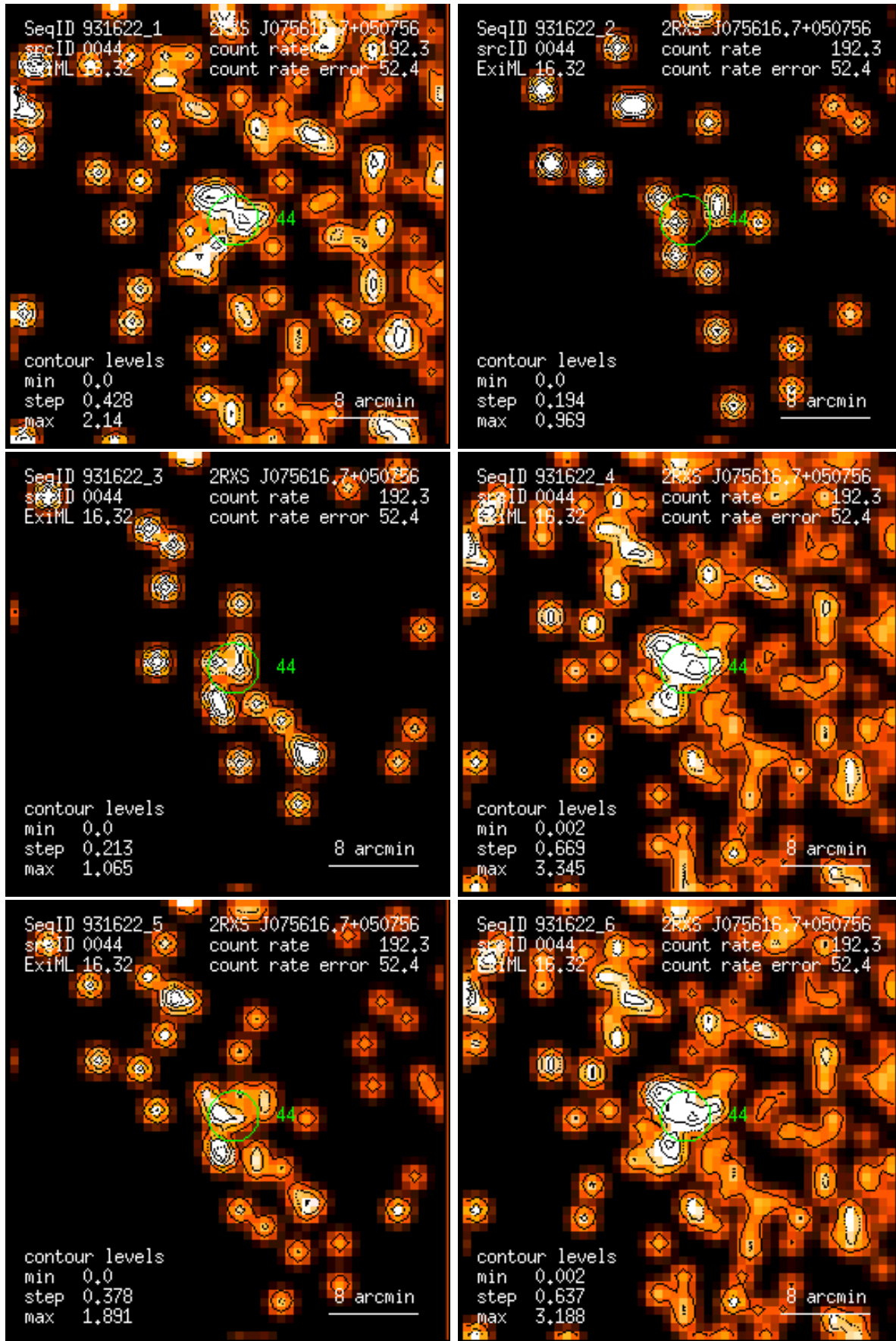
Figure 44: RASS 931622: detection 0044: band rate images, Gaussian filter: (1) PSPC channels 11 – 41, (2) 52 – 90, (3) 91 – 201, (4) 11 – 235, (5) 52 – 201, (6) 11 – 201. Broad band rates in counts/ks. Band rate contour levels in counts/ks/arcmin 2 .
