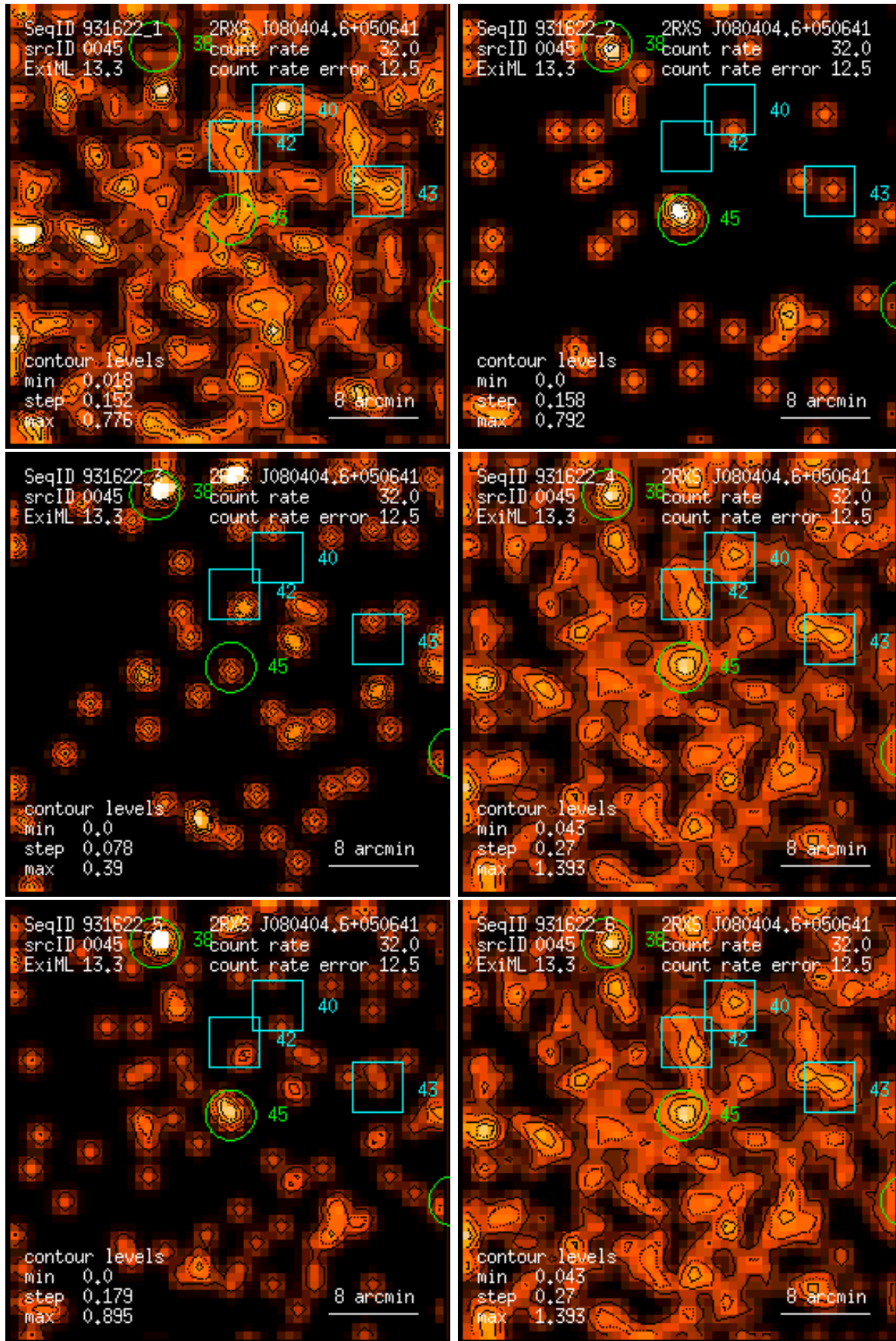
Figure 45: RASS 931622: detection 0045: band rate images, Gaussian filter: (1) PSPC channels 11 – 41, (2) 52 – 90, (3) 91 – 201, (4) 11 – 235, (5) 52 – 201, (6) 11 – 201. Broad band rates in counts/ks. Band rate contour levels in counts/ks/arcmin 2 .
