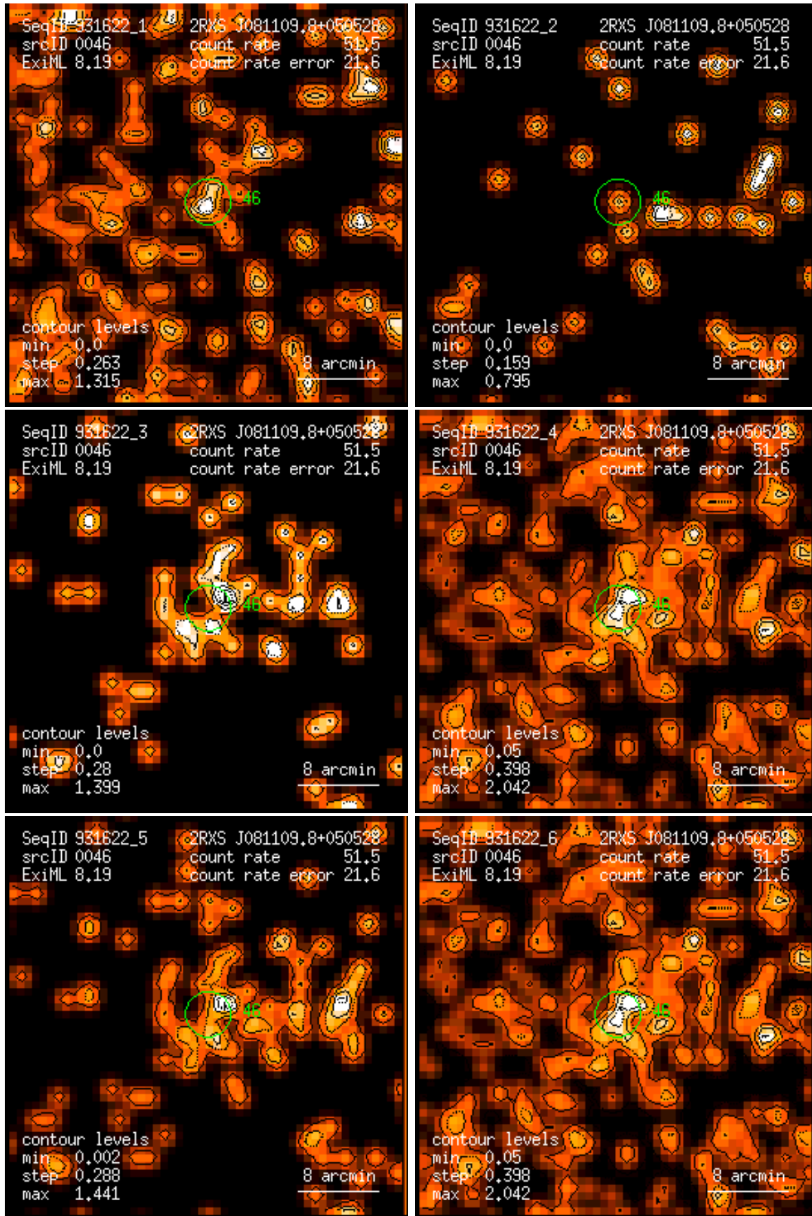
Figure 46: RASS 931622: detection 0046: band rate images, Gaussian filter: (1) PSPC channels 11 – 41, (2) 52 – 90, (3) 91 – 201, (4) 11 – 235, (5) 52 – 201, (6) 11 – 201. Broad band rates in counts/ks. Band rate contour levels in counts/ks/arcmin 2 .
