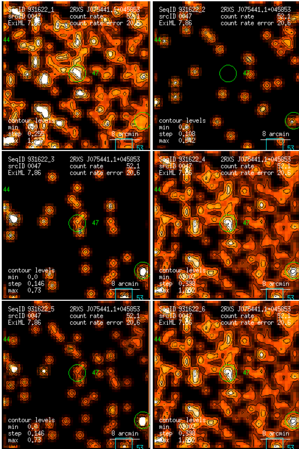
Figure 47: RASS 931622: detection 0047: band rate images, Gaussian filter: (1) PSPC channels 11 – 41, (2) 52 – 90, (3) 91 – 201, (4) 11 – 235, (5) 52 – 201, (6) 11 – 201. Broad band rates in counts/ks. Band rate contour levels in counts/ks/arcmin 2 .
