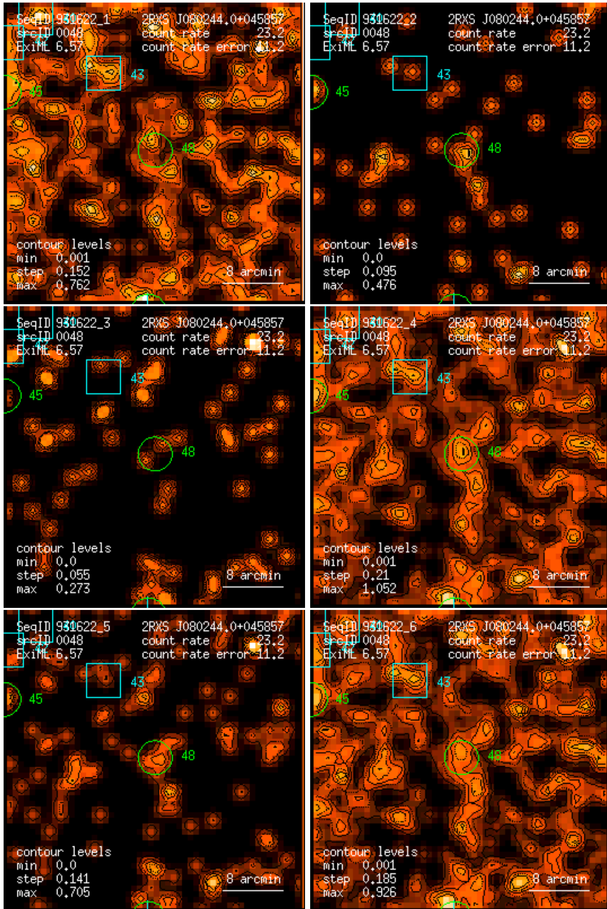
Figure 48: RASS 931622: detection 0048: band rate images, Gaussian filter: (1) PSPC channels 11 – 41, (2) 52 – 90, (3) 91 – 201, (4) 11 – 235, (5) 52 – 201, (6) 11 – 201. Broad band rates in counts/ks. Band rate contour levels in counts/ks/arcmin 2 .
