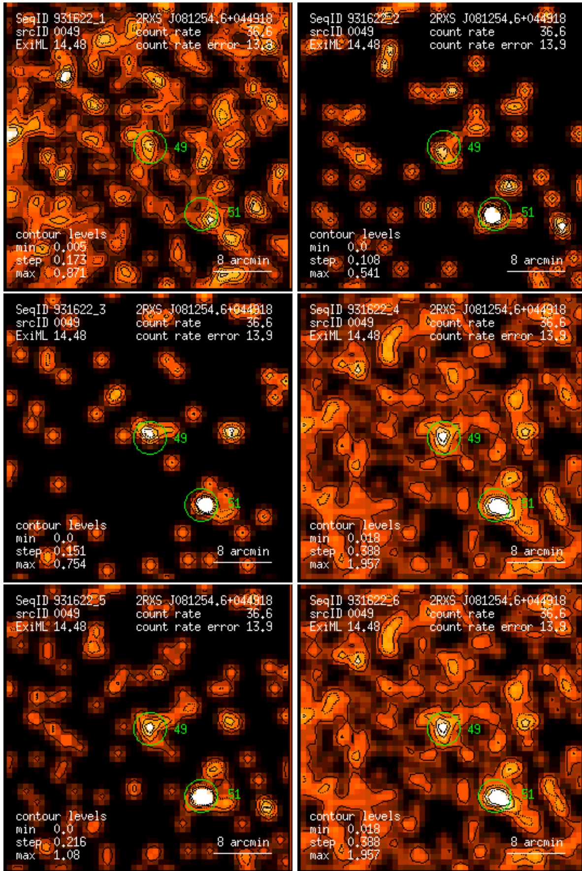
Figure 49: RASS 931622: detection 0049: band rate images, Gaussian filter: (1) PSPC channels 11 – 41, (2) 52 – 90, (3) 91 – 201, (4) 11 – 235, (5) 52 – 201, (6) 11 – 201. Broad band rates in counts/ks. Band rate contour levels in counts/ks/arcmin 2 .
