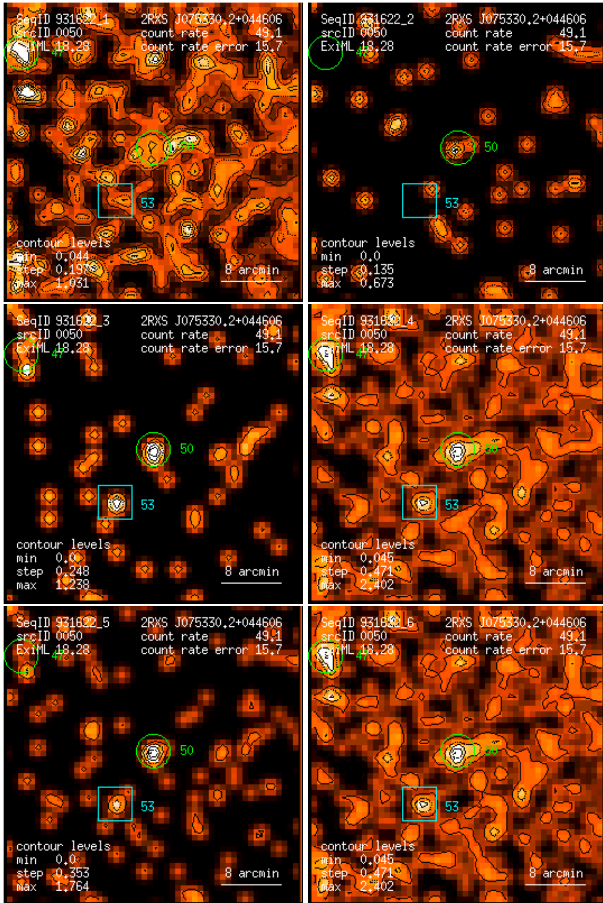
Figure 50: RASS 931622: detection 0050: band rate images, Gaussian filter: (1) PSPC channels 11 – 41, (2) 52 – 90, (3) 91 – 201, (4) 11 – 235, (5) 52 – 201, (6) 11 – 201. Broad band rates in counts/ks. Band rate contour levels in counts/ks/arcmin 2 .
