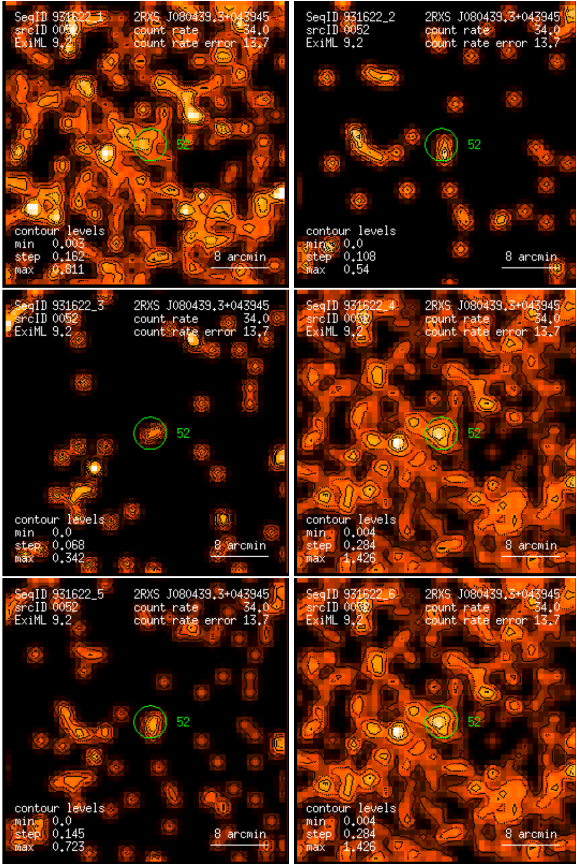
Figure 52: RASS 931622: detection 0052: band rate images, Gaussian filter: (1) PSPC channels 11 – 41, (2) 52 – 90, (3) 91 – 201, (4) 11 – 235, (5) 52 – 201, (6) 11 – 201. Broad band rates in counts/ks. Band rate contour levels in counts/ks/arcmin 2 .
