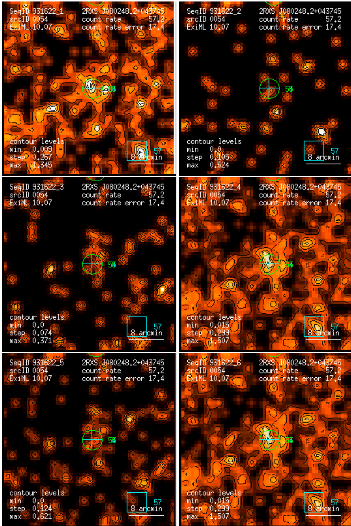
Figure 54: RASS 931622: detection 0054: band rate images, Gaussian filter: (1) PSPC channels 11 – 41, (2) 52 – 90, (3) 91 – 201, (4) 11 – 235, (5) 52 – 201, (6) 11 – 201. Broad band rates in counts/ks. Band rate contour levels in counts/ks/arcmin 2 .
