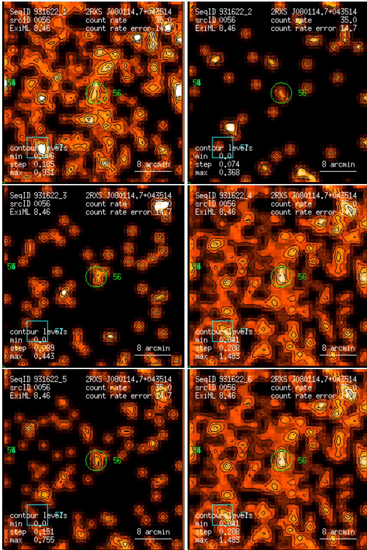
Figure 56: RASS 931622: detection 0056: band rate images, Gaussian filter: (1) PSPC channels 11 – 41, (2) 52 – 90, (3) 91 – 201, (4) 11 – 235, (5) 52 – 201, (6) 11 – 201. Broad band rates in counts/ks. Band rate contour levels in counts/ks/arcmin 2 .
