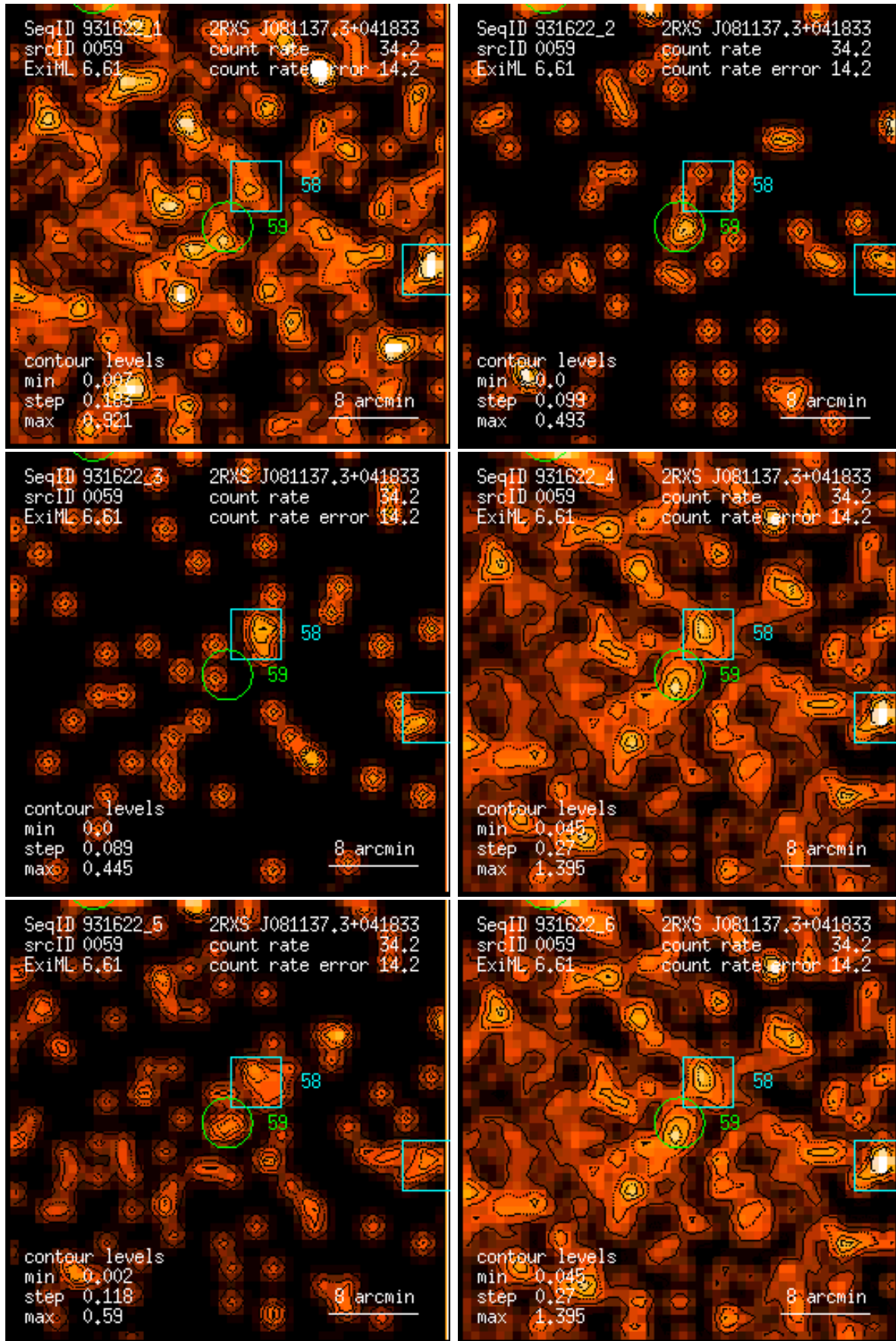
Figure 59: RASS 931622: detection 0059: band rate images, Gaussian filter: (1) PSPC channels 11 – 41, (2) 52 – 90, (3) 91 – 201, (4) 11 – 235, (5) 52 – 201, (6) 11 – 201. Broad band rates in counts/ks. Band rate contour levels in counts/ks/arcmin 2 .
