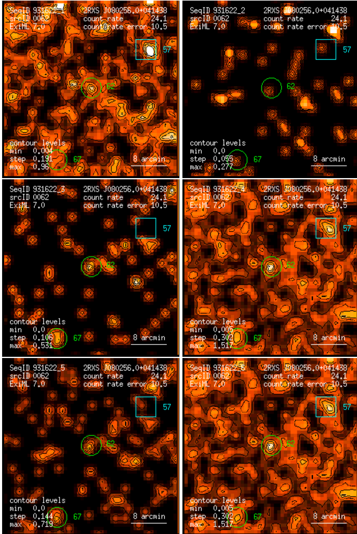
Figure 62: RASS 931622: detection 0062: band rate images, Gaussian filter: (1) PSPC channels 11 – 41, (2) 52 – 90, (3) 91 – 201, (4) 11 – 235, (5) 52 – 201, (6) 11 – 201. Broad band rates in counts/ks. Band rate contour levels in counts/ks/arcmin 2 .
