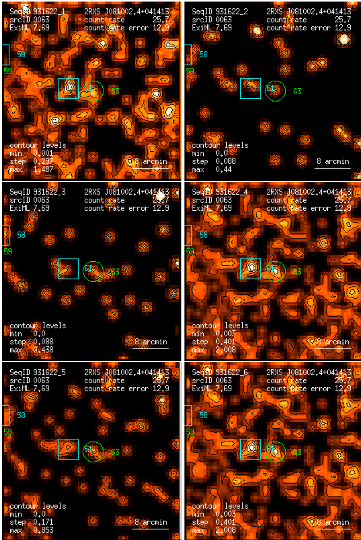
Figure 63: RASS 931622: detection 0063: band rate images, Gaussian filter: (1) PSPC channels 11 – 41, (2) 52 – 90, (3) 91 – 201, (4) 11 – 235, (5) 52 – 201, (6) 11 – 201. Broad band rates in counts/ks. Band rate contour levels in counts/ks/arcmin 2 .
