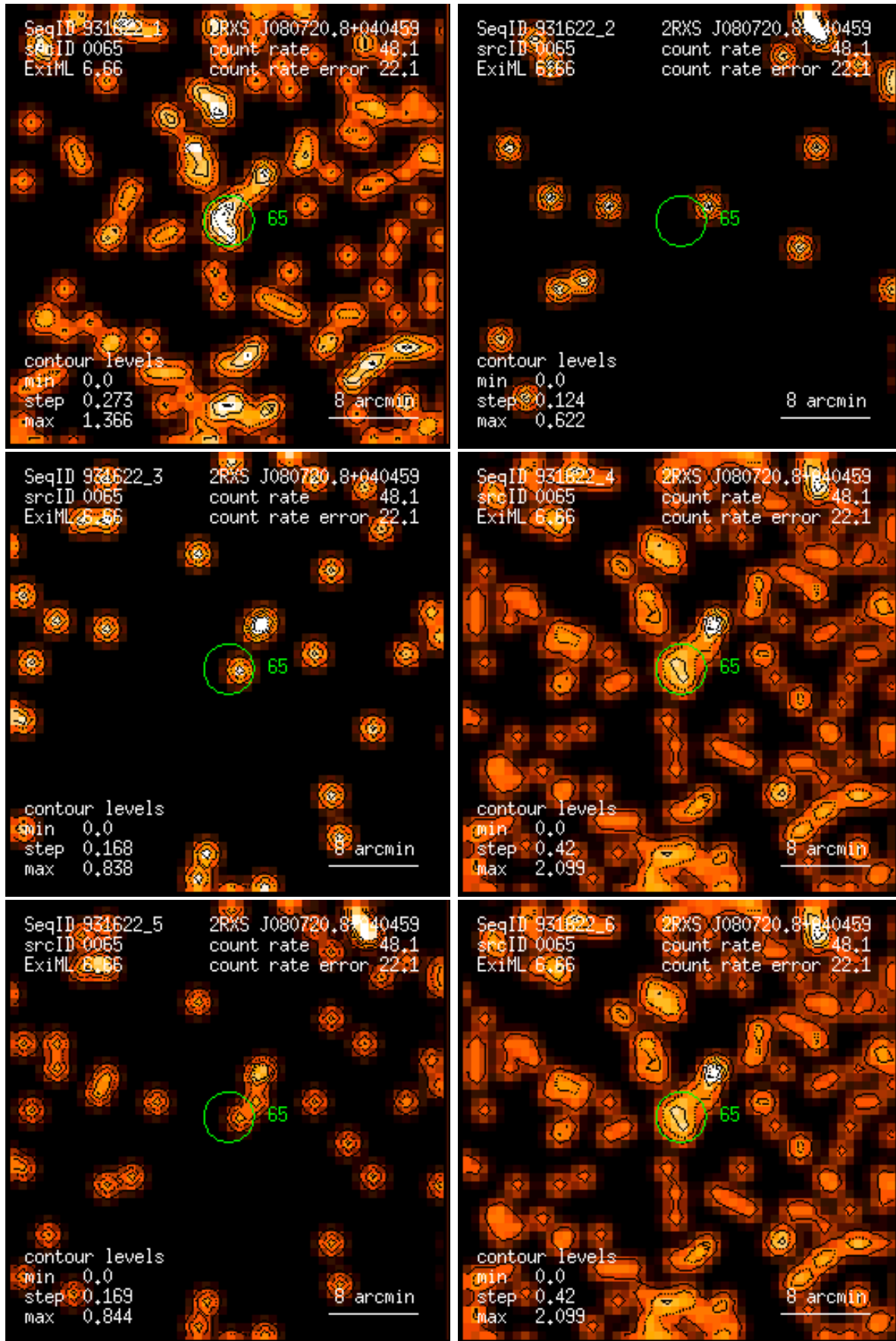
Figure 65: RASS 931622: detection 0065: band rate images, Gaussian filter: (1) PSPC channels 11 – 41, (2) 52 – 90, (3) 91 – 201, (4) 11 – 235, (5) 52 – 201, (6) 11 – 201. Broad band rates in counts/ks. Band rate contour levels in counts/ks/arcmin 2 .
