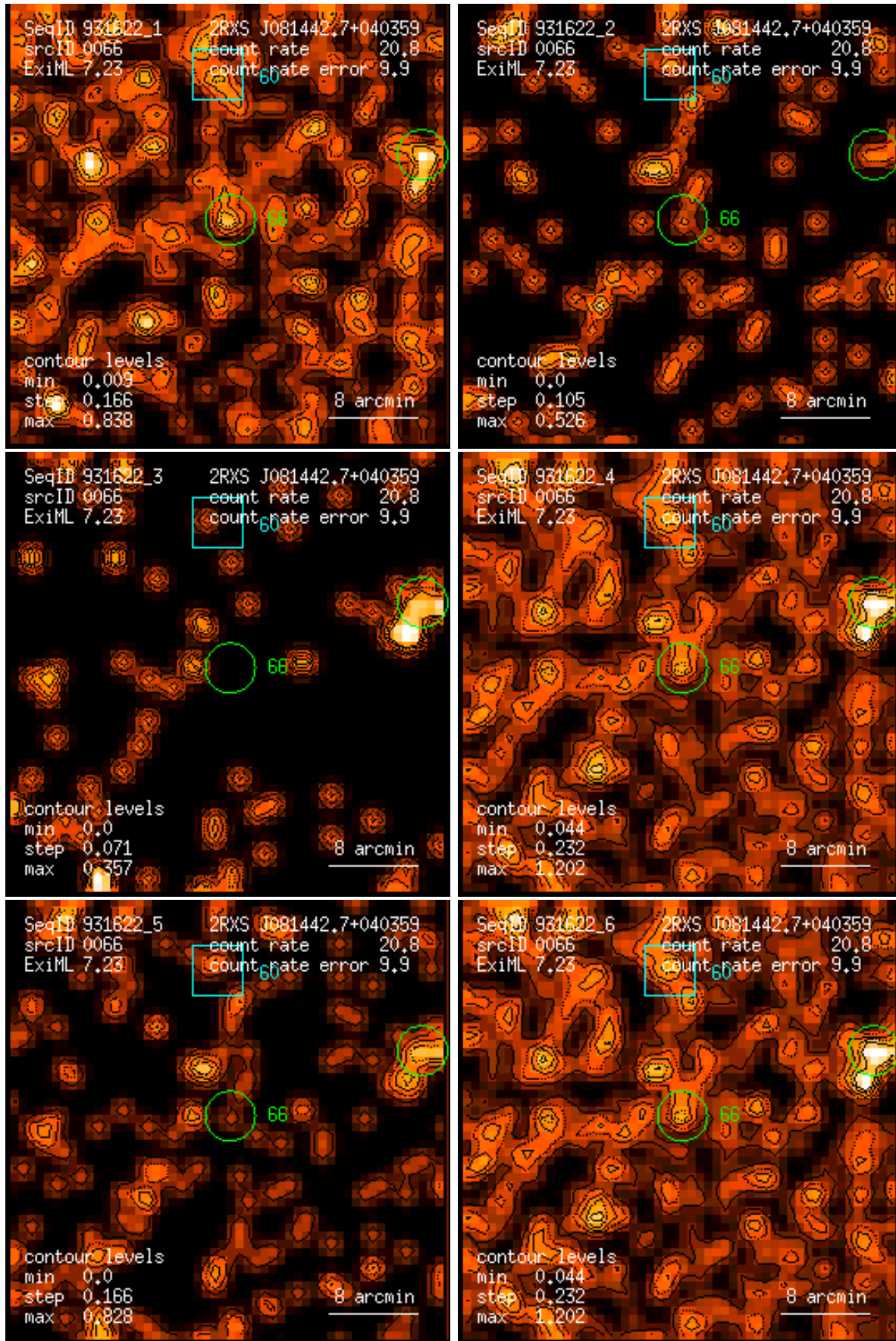
Figure 66: RASS 931622: detection 0066: band rate images, Gaussian filter: (1) PSPC channels 11 – 41, (2) 52 – 90, (3) 91 – 201, (4) 11 – 235, (5) 52 – 201, (6) 11 – 201. Broad band rates in counts/ks. Band rate contour levels in counts/ks/arcmin 2 .
