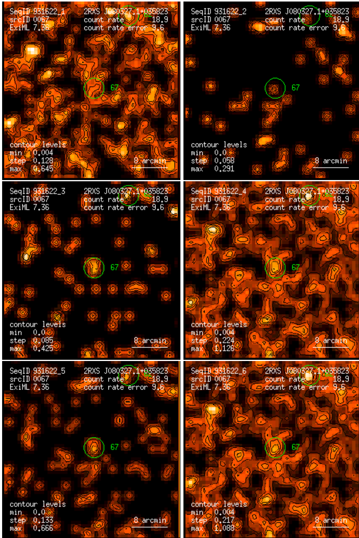
Figure 67: RASS 931622: detection 0067: band rate images, Gaussian filter: (1) PSPC channels 11 – 41, (2) 52 – 90, (3) 91 – 201, (4) 11 – 235, (5) 52 – 201, (6) 11 – 201. Broad band rates in counts/ks. Band rate contour levels in counts/ks/arcmin 2 .
