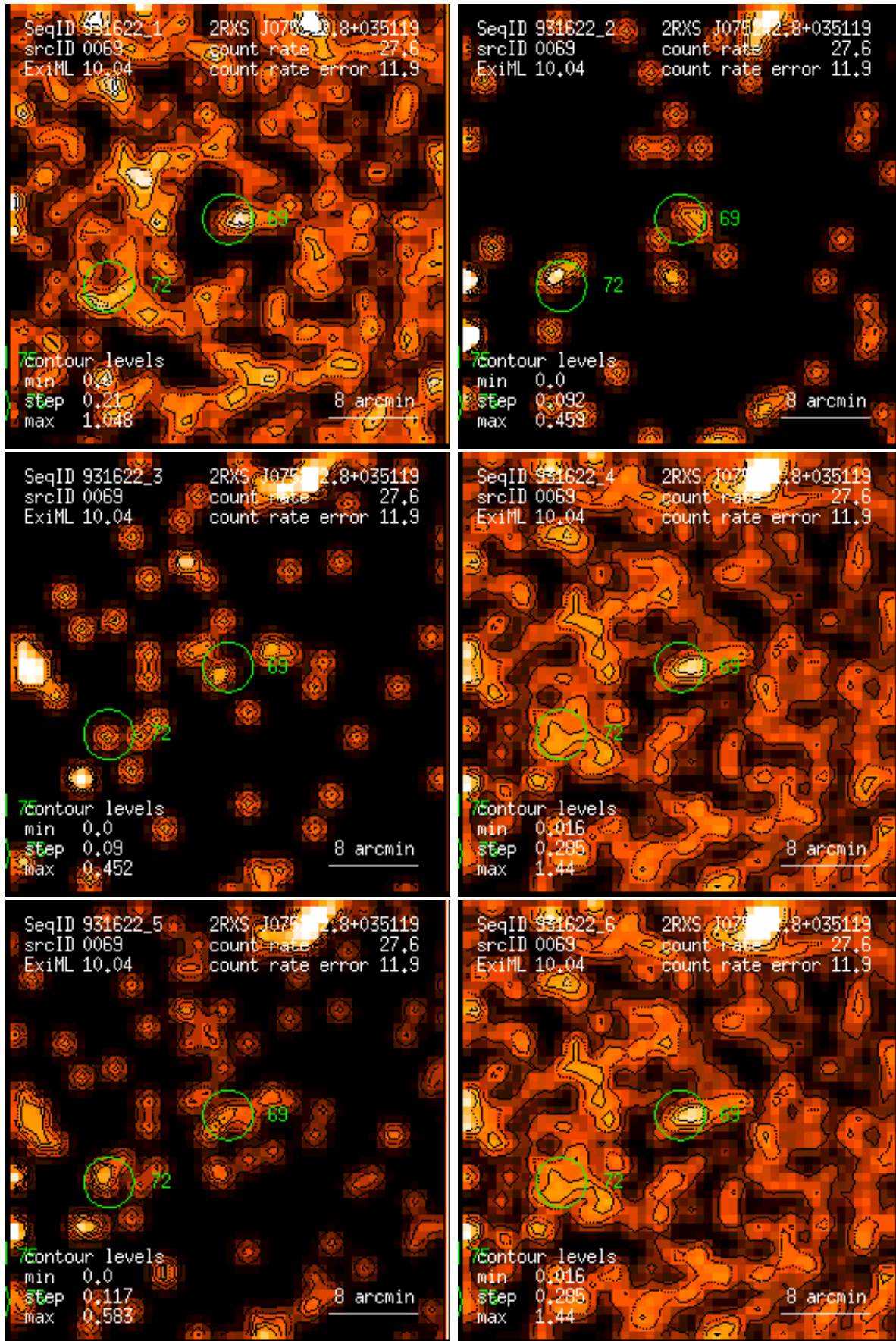
Figure 69: RASS 931622: detection 0069: band rate images, Gaussian filter: (1) PSPC channels 11 – 41, (2) 52 – 90, (3) 91 – 201, (4) 11 – 235, (5) 52 – 201, (6) 11 – 201. Broad band rates in counts/ks. Band rate contour levels in counts/ks/arcmin 2 .
