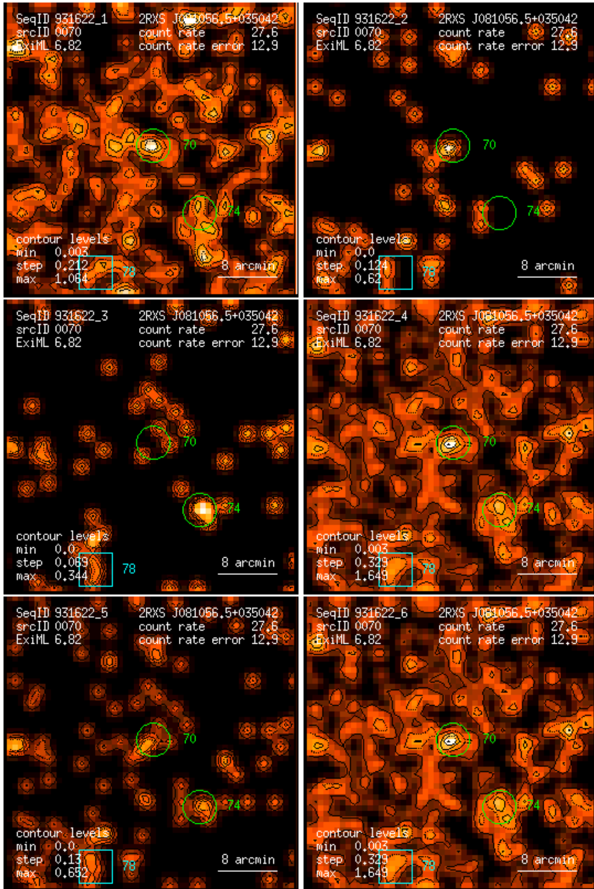
Figure 70: RASS 931622: detection 0070: band rate images, Gaussian filter: (1) PSPC channels 11 – 41, (2) 52 – 90, (3) 91 – 201, (4) 11 – 235, (5) 52 – 201, (6) 11 – 201. Broad band rates in counts/ks. Band rate contour levels in counts/ks/arcmin 2 .
